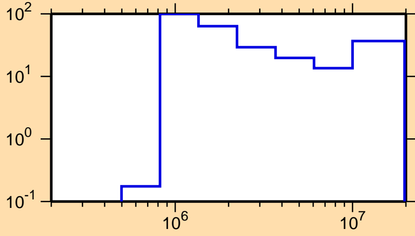
\Delta\sigma/\sigma vs. E for ^{82}\text{Rb}(n,ncont.)
