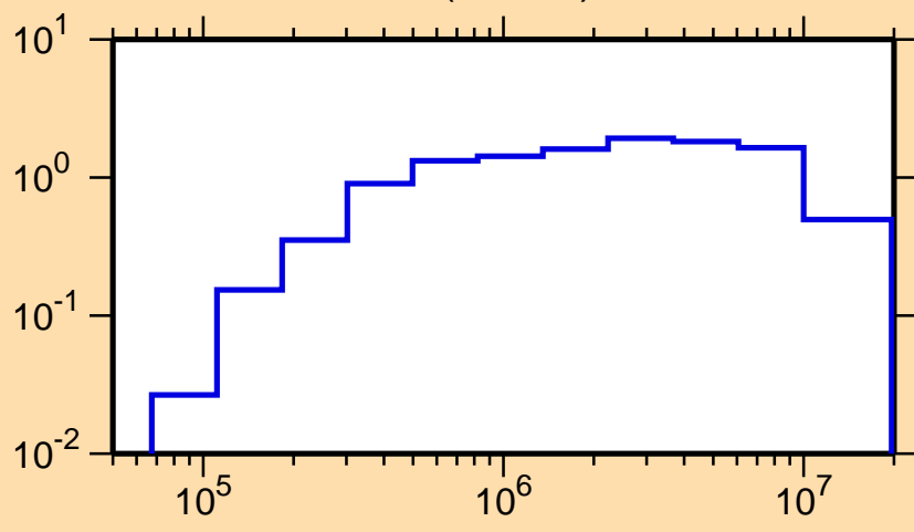
\sigma vs. E for ^{82}\text{Rb}(n,\text{inel.})
