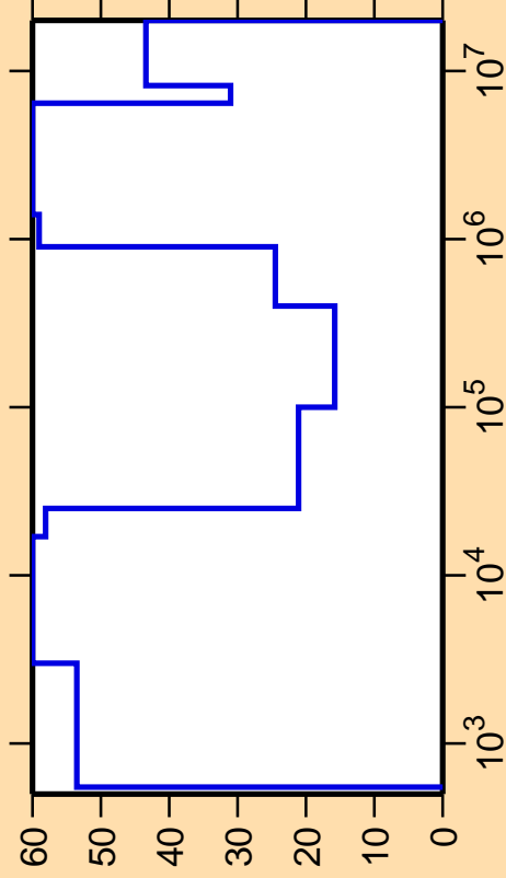
\Delta\sigma/\sigma vs. E for ^{82}\text{Rb}(n,p)
