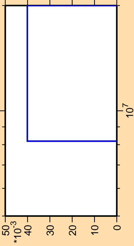
\Delta\sigma/\sigma vs. E for ^{82}\text{Rb} (mt 34)
