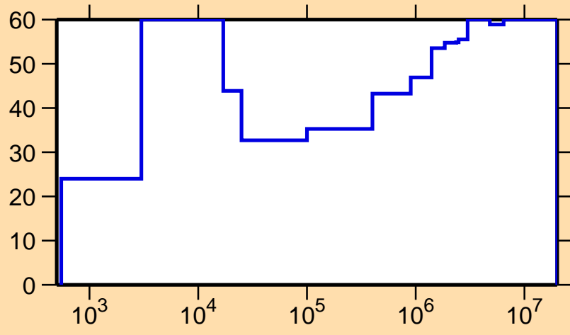
\Delta\sigma/\sigma vs. E for ^{82}\text{Rb}(n,\gamma)
