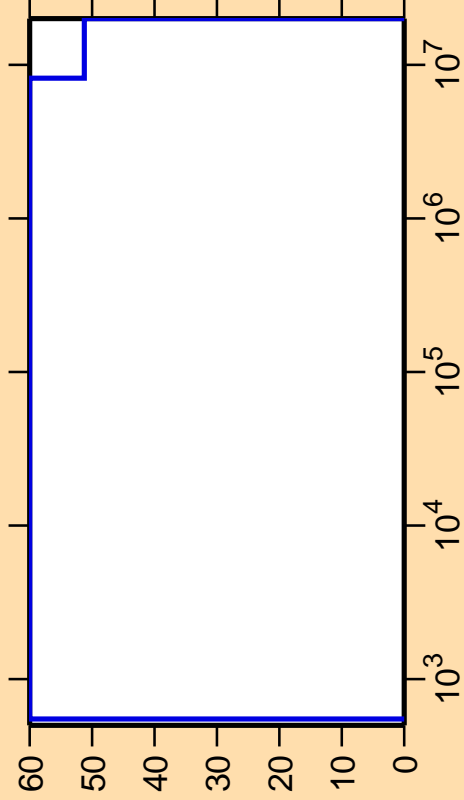
\Delta\sigma/\sigma vs. E for ^{82}\text{Rb}(n,\alpha)
