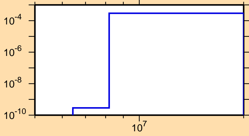
\sigma vs. E for ^{82}\text{Rb}(n,t)
