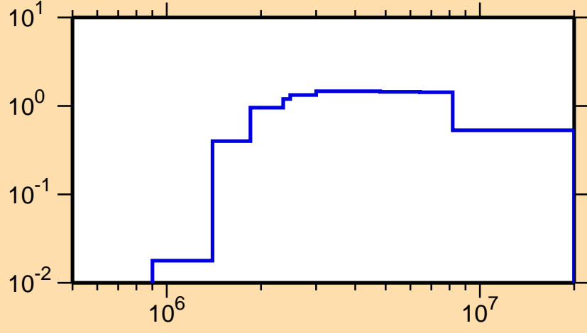
\sigma vs. E for ^{82}\text{Rb}(n,n\text{cont.})
