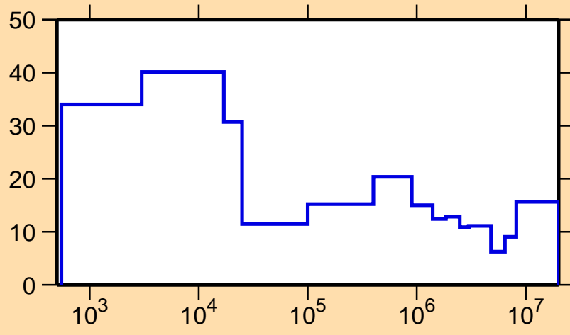
\Delta\sigma/\sigma vs. E for ^{82}\text{Rb}(n,el.)
