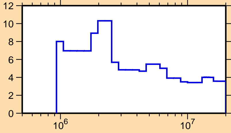
\Delta\sigma/\sigma vs. E for ^{82}\text{Rb}(n,n\text{nonel.})
