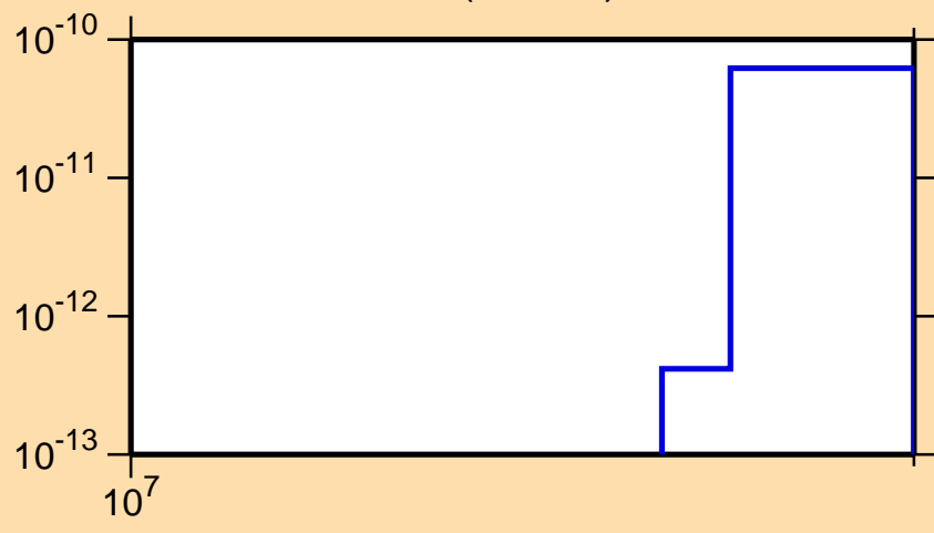
\sigma vs. E for ^{82}\text{Rb}(\text{mt117})
