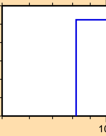
\sigma vs. E for ^{82}\text{Rb} (mt 34)
