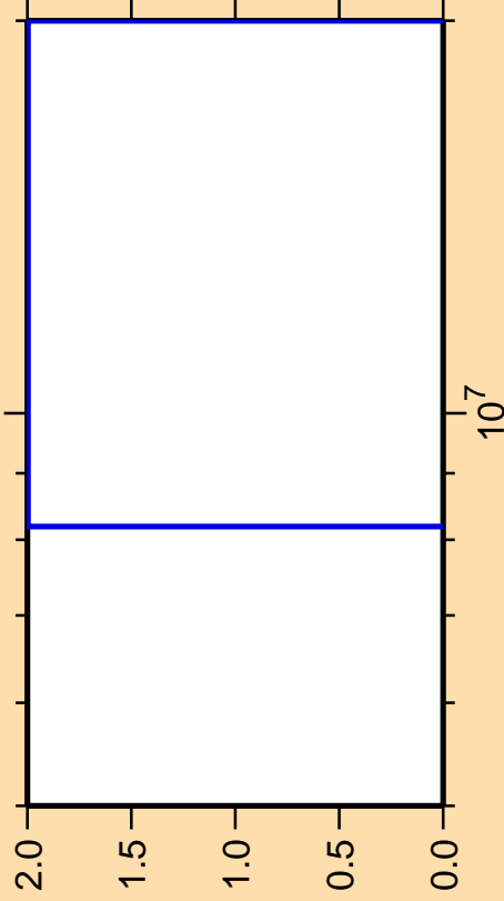
\Delta\sigma/\sigma vs. E for ^{82}\text{Rb}(n,\text{pt})
