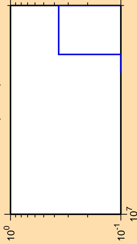
\Delta\sigma/\sigma vs. E for ^{83}\text{Rb}(n,2n\alpha)
