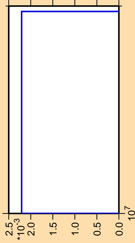
\Delta\sigma/\sigma vs. E for ^{83}\text{Rb}(n,2n\alpha)
