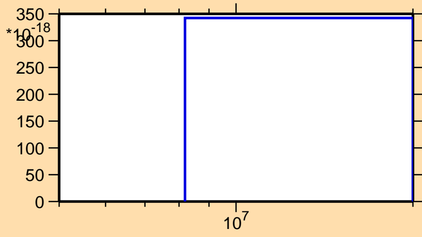
\sigma vs. E for ^{83}\text{Rb}(n,2n\alpha)
