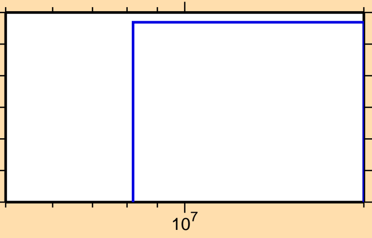
\sigma vs. E for ^{83}\text{Rb}(n,p\alpha)
