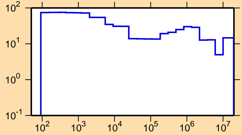
\Delta\sigma/\sigma vs. E for ^{84}\text{Rb}(n,\text{el.})
