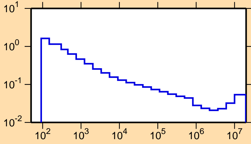
\sigma vs. E for ^{84}\text{Rb}(n,p)
