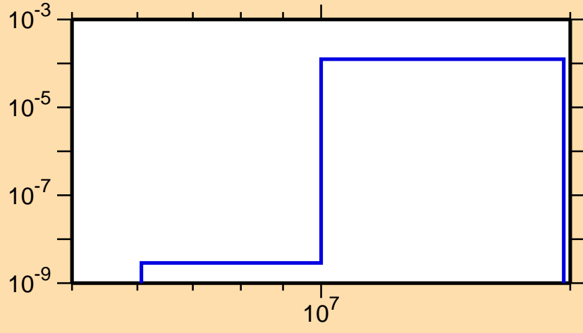
\sigma vs. E for ^{84}\text{Rb}(n,t)
