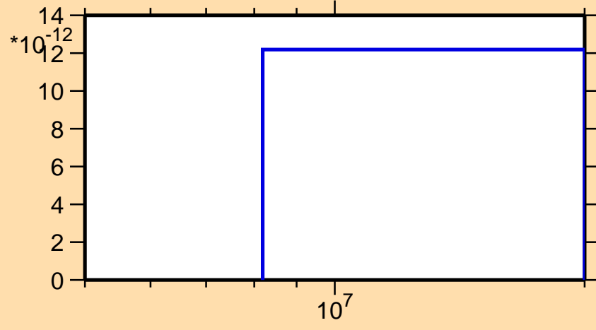
\sigma vs. E for ^{84}\text{Rb}(n,3n)
