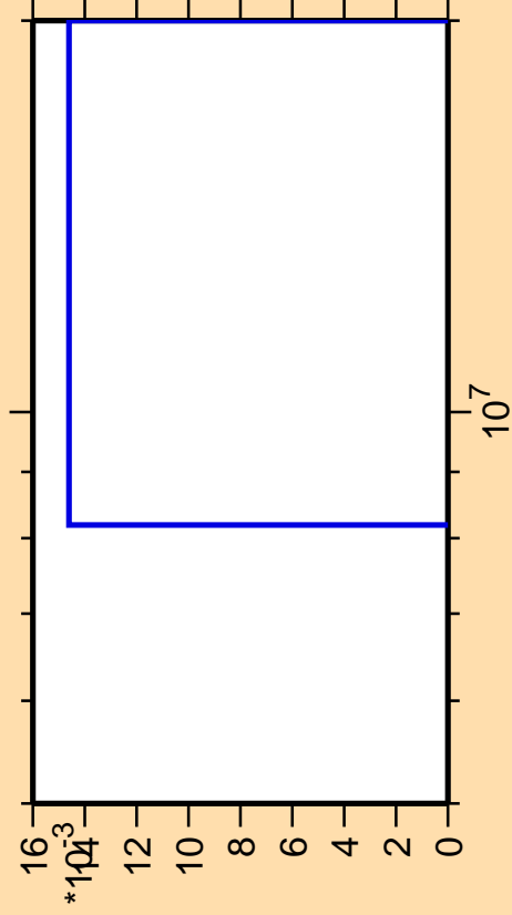
\Delta\sigma/\sigma vs. E for ^{84}\text{Rb}(n,\text{pd})
