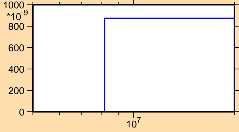
\sigma vs. E for ^{84}\text{Rb}(n,\text{nd})
