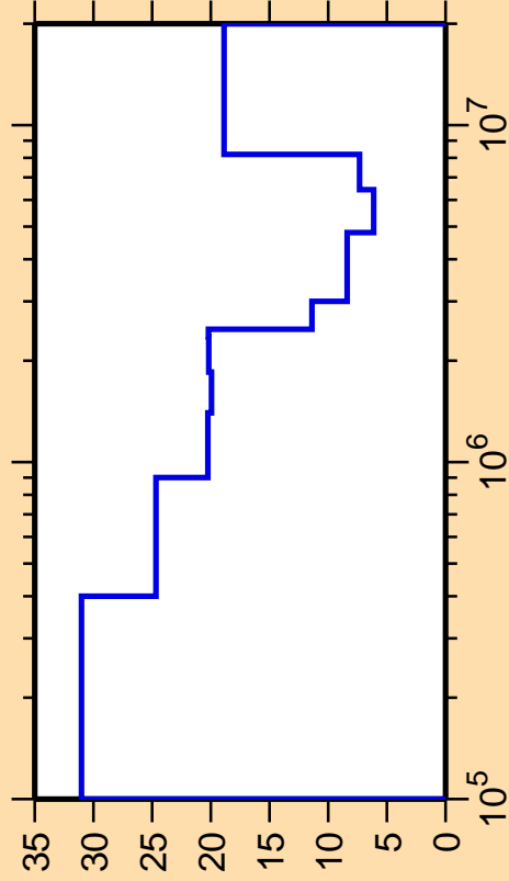
\Delta\sigma/\sigma vs. E for ^{84}\text{Rb}(n,\text{inel.})
