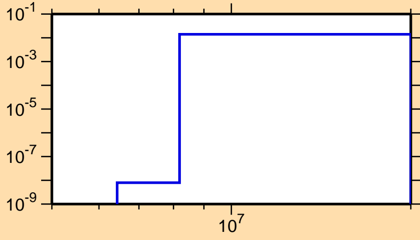
\sigma vs. E for ^{84}\text{Rb}(n,np)
