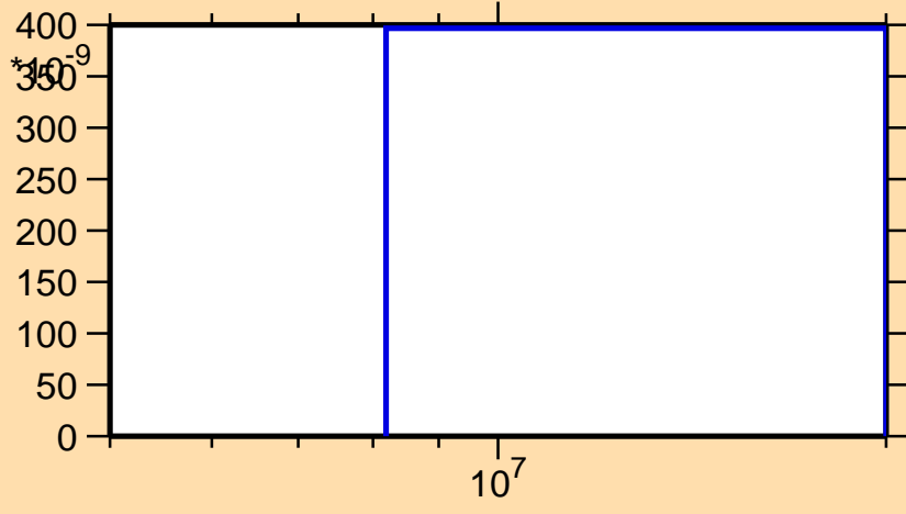
\sigma vs. E for ^{84}\text{Rb}(n,p\alpha)
