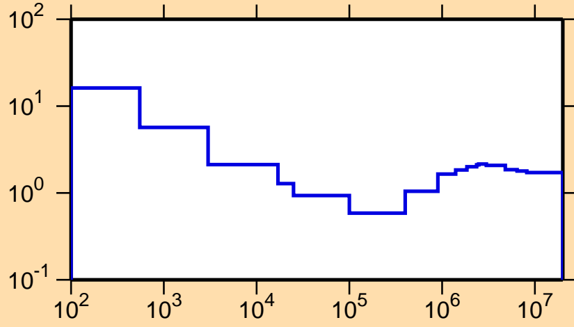
\sigma vs. E for ^{84}\text{Rb}(n,\text{nonel.})
