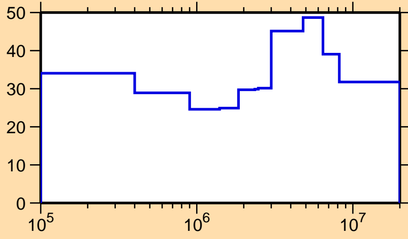
\Delta\sigma/\sigma vs. E for ^{84}\text{Rb}(n,n_1)
