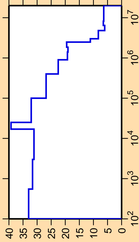
\Delta\sigma/\sigma vs. E for ^{84}\text{Rb}(n,\text{nonel.})
