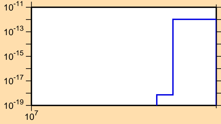
\sigma vs. E for ^{84}\text{Rb}(n,\text{pd})
