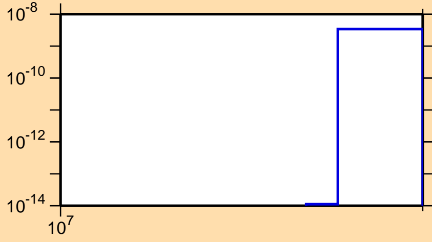
\sigma vs. E for ^{84}\text{Rb}(n,2n\alpha)
