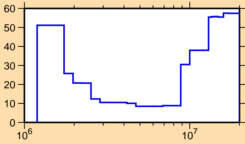
\Delta\sigma/\sigma vs. E for ^{84}\text{Rb}(n,ncont.)
