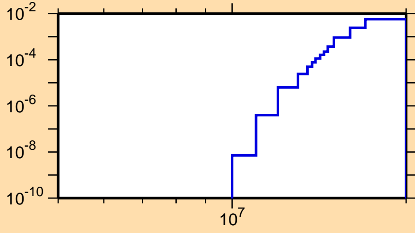
\sigma vs. E for ^{84}\text{Rb}(n,n\alpha)
