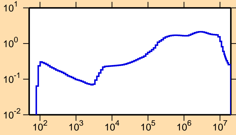
\sigma vs. E for ^{84}\text{Rb}(n,\text{inel.})
