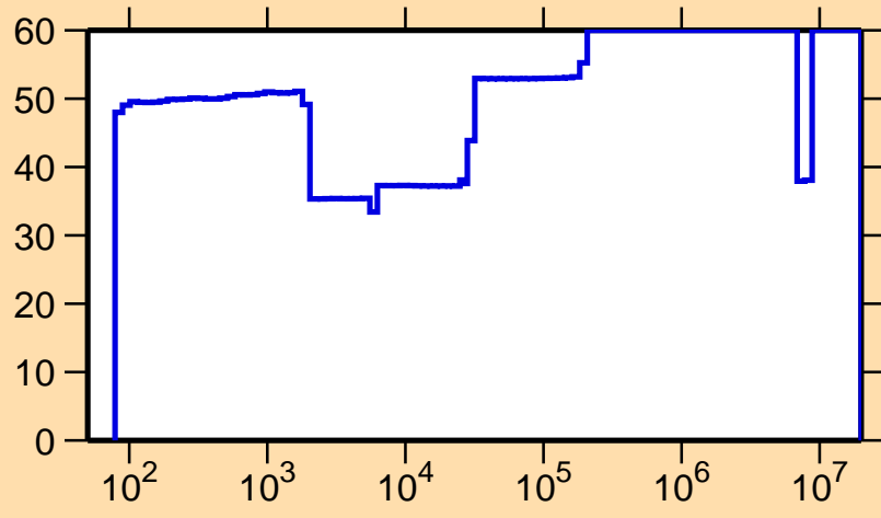
\Delta\sigma/\sigma vs. E for ^{84}\text{Rb}(n,\gamma)
