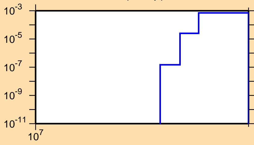
\sigma vs. E for ^{84}\text{Rb}(n,2np)
