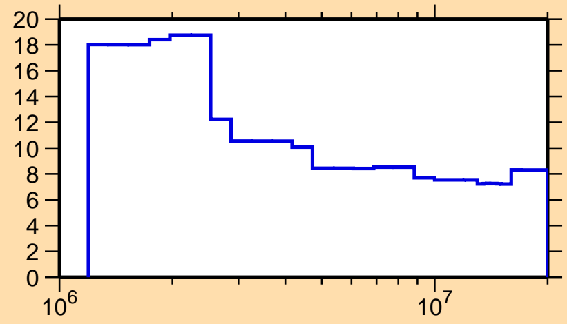
\Delta\sigma/\sigma vs. E for ^{84}\text{Rb}(n,n\text{onel.})
