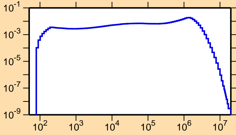
\sigma vs. E for ^{84}\text{Rb}(n,n_1)
