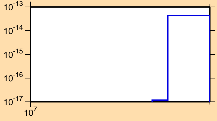
\sigma vs. E for ^{84}\text{Rb}(\text{mt117})
