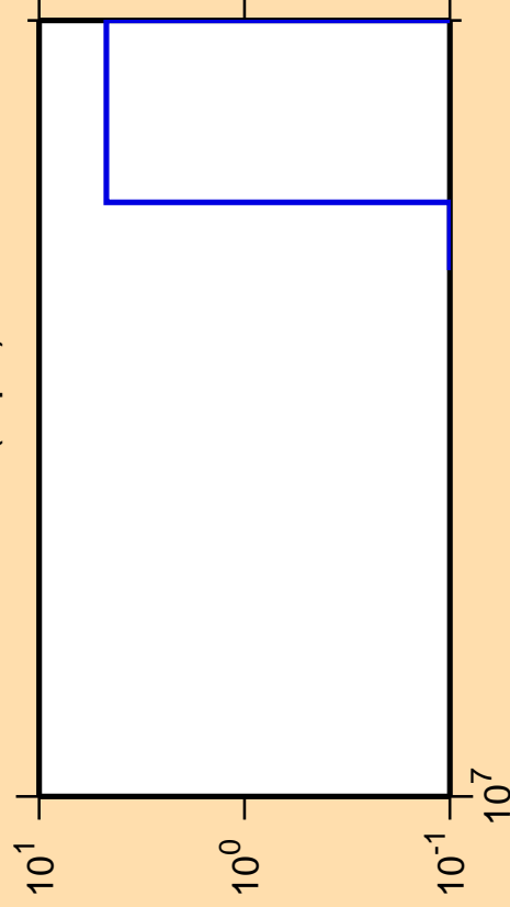
\Delta\sigma/\sigma vs. E for ^{84}\text{Rb}(n,\text{pd})
