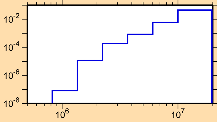
\sigma vs. E for ^{85}\text{Rb}(n,p)
