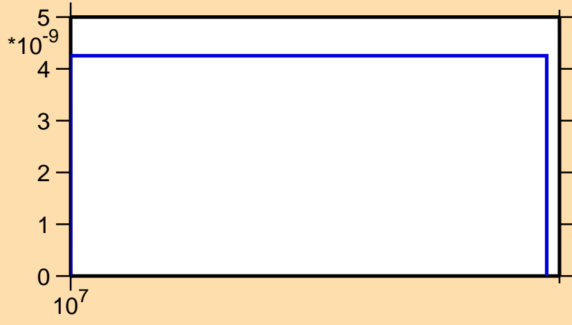
\sigma vs. E for ^{85}\text{Rb}(n,nd)
