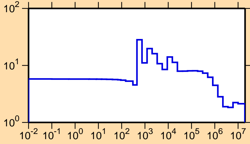
\sigma vs. E for ^{85}\text{Rb}(n,\text{el.})
