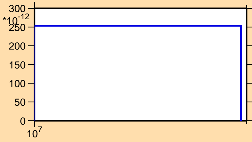
\sigma vs. E for ^{85}\text{Rb}(n,2np)
