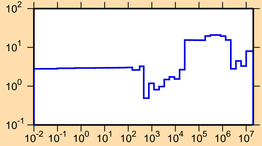
\Delta\sigma/\sigma vs. E for ^{85}\text{Rb}(n,\text{tot.})
