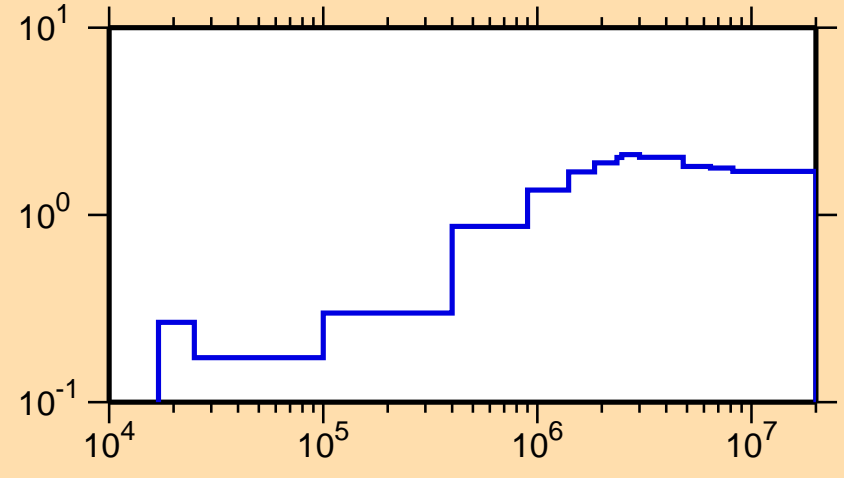
\sigma vs. E for ^{85}\text{Rb}(n,\text{nonel.})
