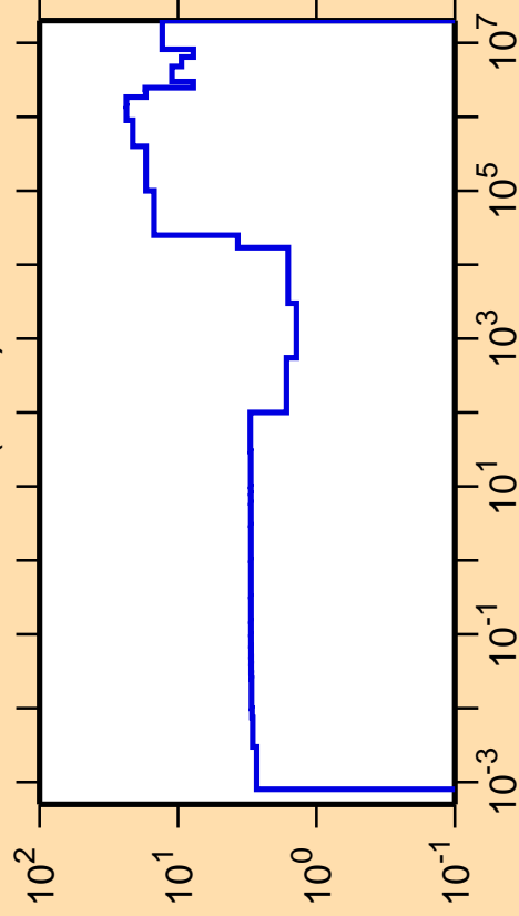
\Delta\sigma/\sigma vs. E for ^{85}\text{Rb}(n,\text{el.})
