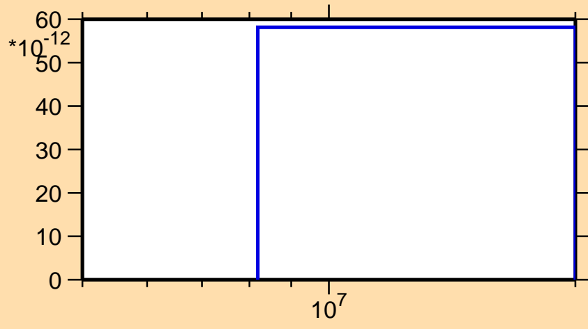
\sigma vs. E for ^{85}\text{Rb}(n,p\alpha)
