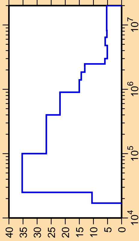
\Delta\sigma/\sigma vs. E for ^{85}\text{Rb}(n,\text{nonel.})
