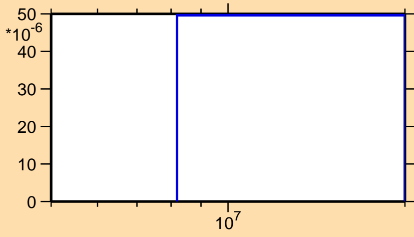
\sigma vs. E for ^{85}\text{Rb}(n,t)
