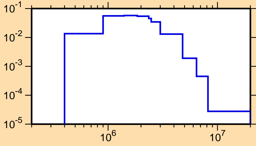
\sigma vs. E for ^{86}\text{Rb}(n,n_2)
