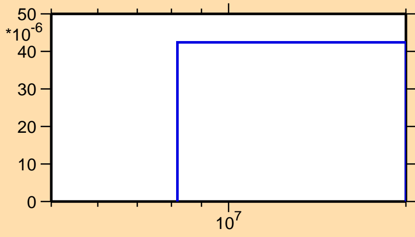
\sigma vs. E for ^{86}\text{Rb}(n,n\alpha)
