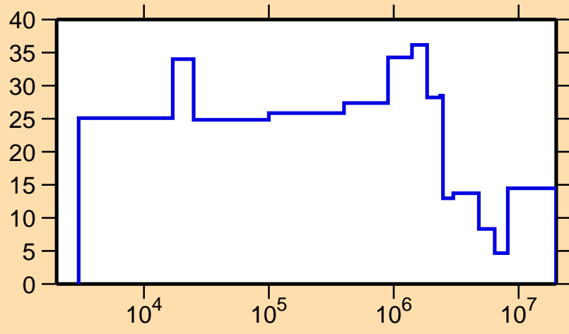
\Delta\sigma/\sigma vs. E for ^{86}\text{Rb}(n,el.)
