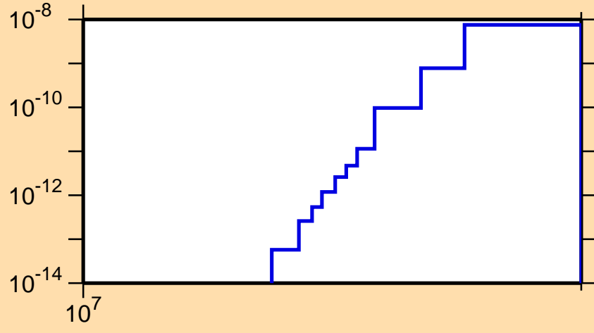
\sigma vs. E for ^{86}\text{Rb}(n,p\alpha)
