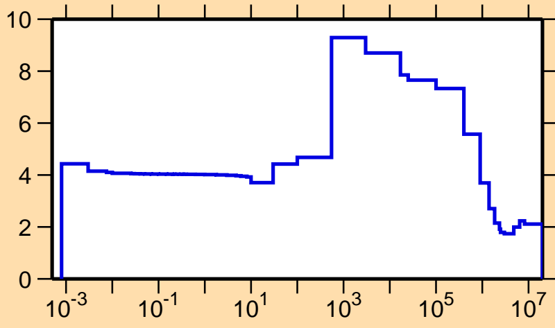
\sigma vs. E for ^{86}\text{Rb}(n,\text{el.})
