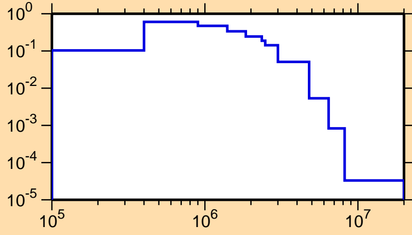
\sigma vs. E for ^{86}\text{Rb}(n,n_4)
