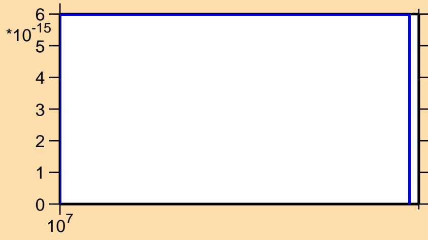
\sigma vs. E for ^{87}\text{Rb}(n,2np)
