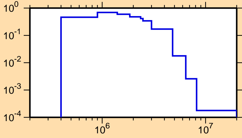
\sigma vs. E for ^{87}\text{Rb}(n,n_1)
