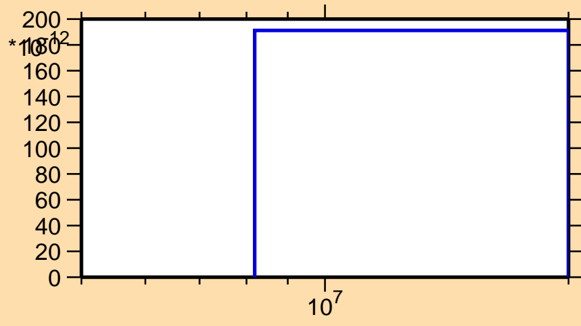
\sigma vs. E for ^{87}\text{Rb}(n,\text{nd})
