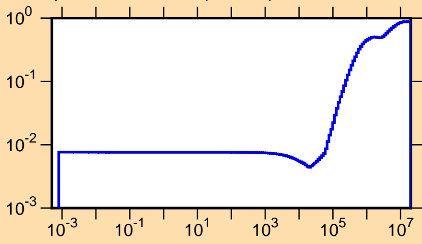
\mu vs. E for ^{88}\text{Rb}(\text{mt251})
