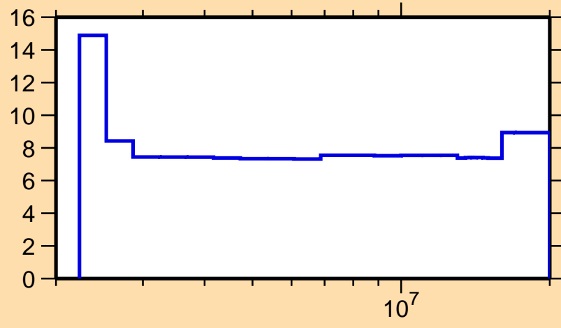
\Delta\sigma/\sigma vs. E for ^{88}\text{Rb}(n,n\text{onel.})
