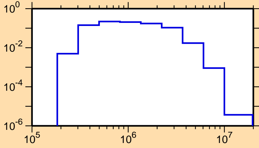
\sigma vs. E for ^{88}\text{Rb}(n,n_3)
