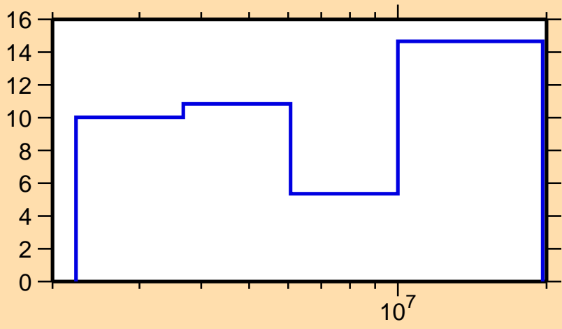
\Delta\sigma/\sigma vs. E for ^{88}\text{Rb}(n,el.)
