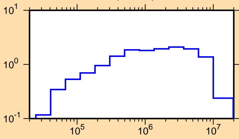
\sigma vs. E for ^{88}\text{Rb}(n,\text{inel.})
