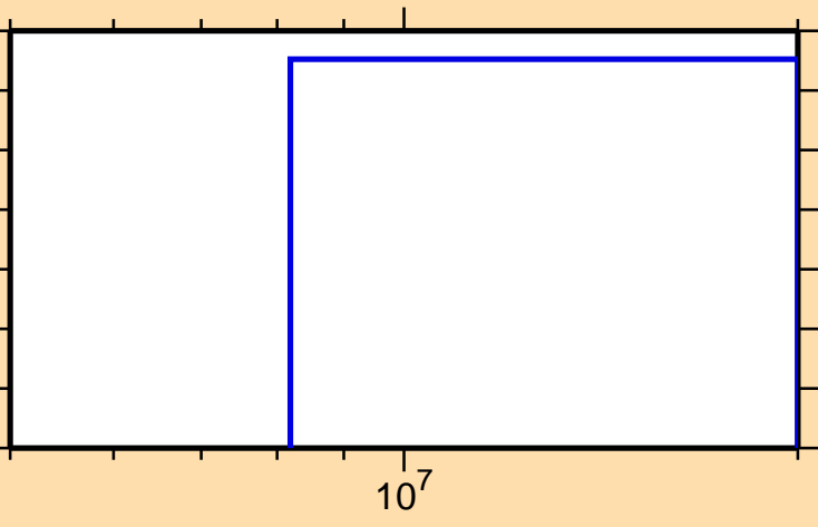
\sigma vs. E for ^{88}\text{Rb}(n,2np)
