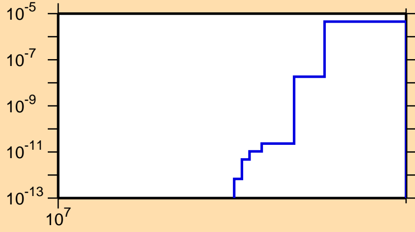
\sigma vs. E for ^{89}\text{Rb}(n,\text{nd})
