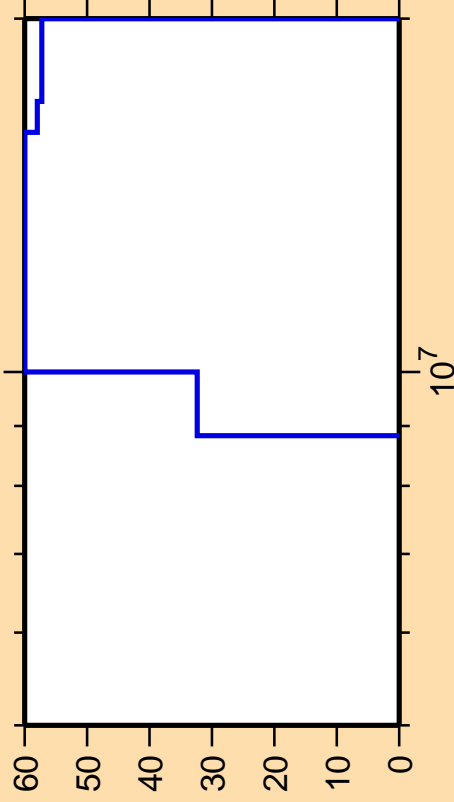
\Delta\sigma/\sigma vs. E for ^{89}\text{Rb}(n,n\alpha)
