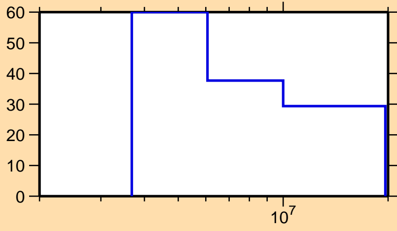
\Delta\sigma/\sigma vs. E for ^{89}\text{Rb}(n,p)
