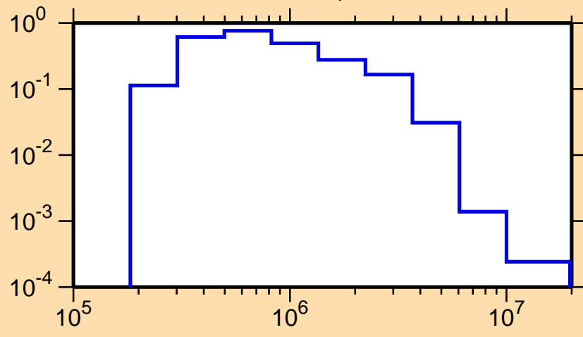
\sigma vs. E for ^{89}\text{Rb}(n,n_1)
