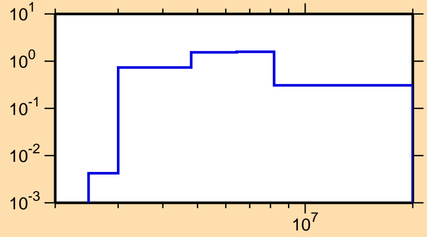
\sigma vs. E for ^{89}\text{Rb}(n,n\text{cont.})
