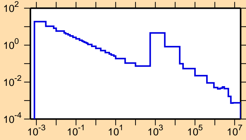
\sigma vs. E for ^{89}\text{Rb}(n,\gamma)
