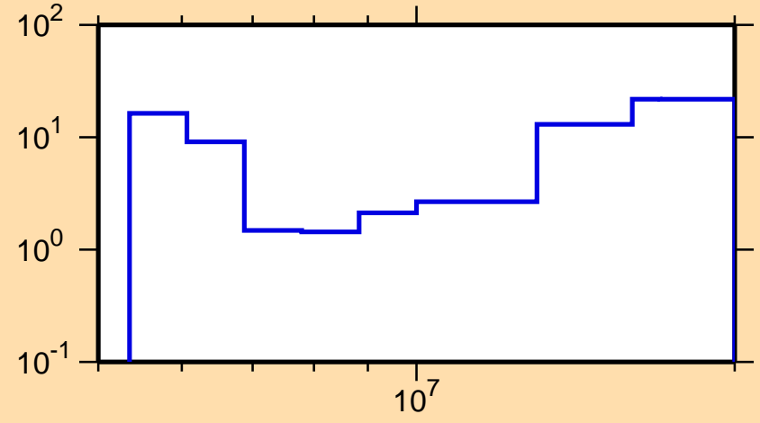
\Delta\sigma/\sigma vs. E for ^{90}\text{Rb}(n,2n)
