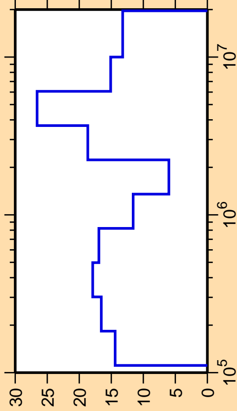
\Delta\sigma/\sigma vs. E for ^{90}\text{Rb}(n,n_2)
