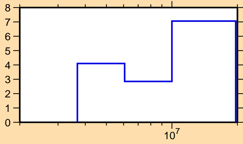
\Delta\sigma/\sigma vs. E for ^{90}\text{Rb}(n,el.)
