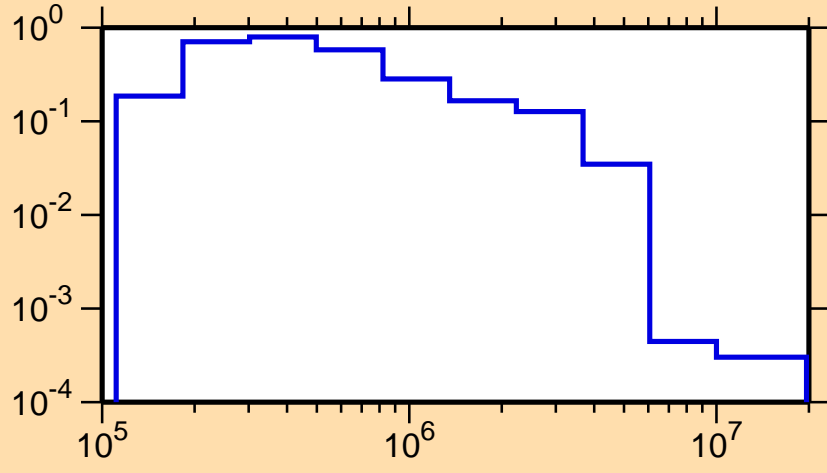
\sigma vs. E for ^{90}\text{Rb}(n,n_2)
