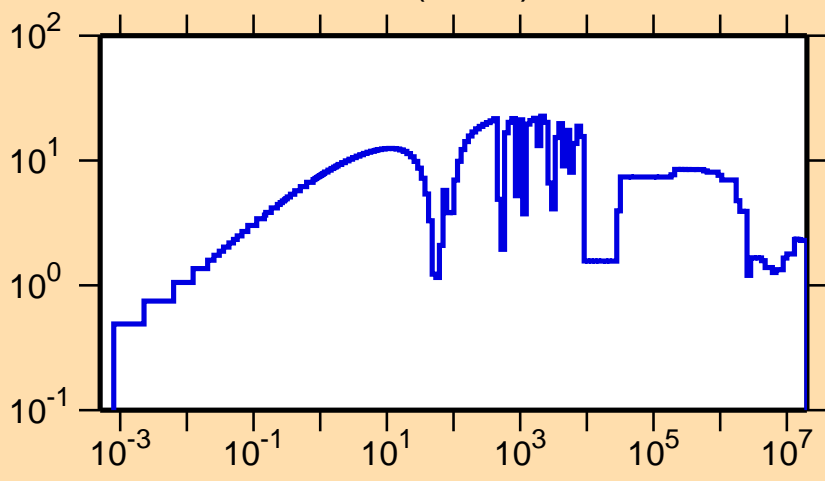
\Delta\sigma/\sigma vs. E for ^{90}\text{Rb}(n,\text{tot.})
