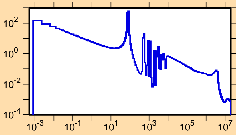
\sigma vs. E for ^{90}\text{Rb}(n,\gamma)
