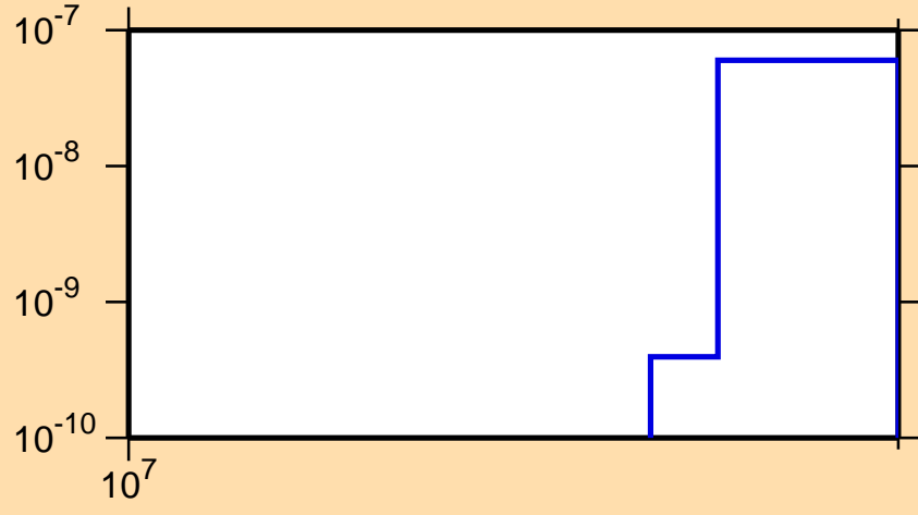
\sigma vs. E for ^{90}\text{Rb}(n,2n\alpha)
