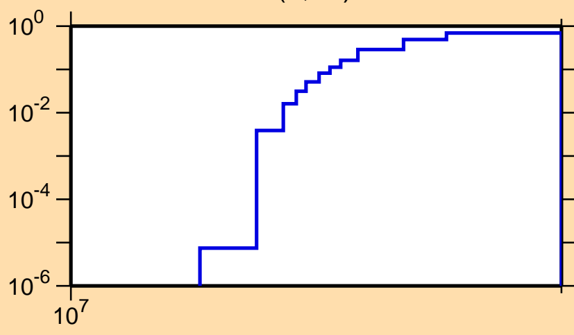
\sigma vs. E for ^{90}\text{Rb}(n,3n)
