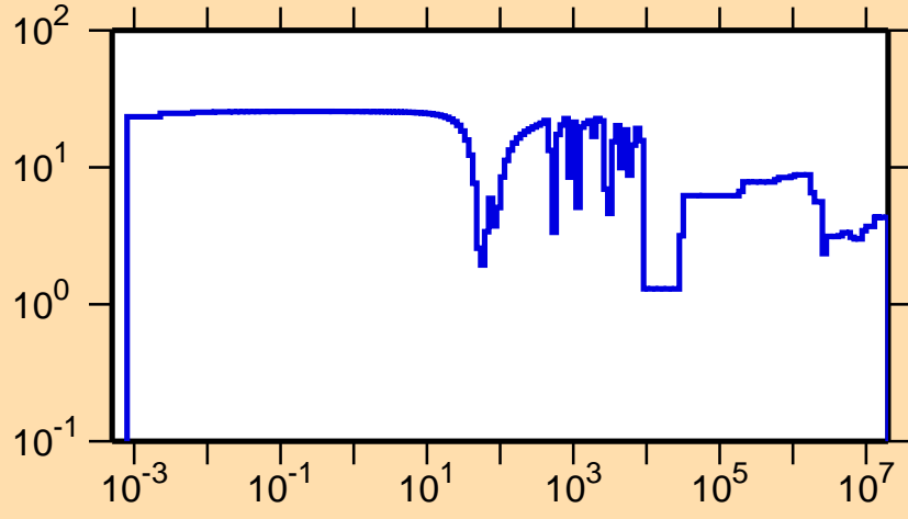
\Delta\sigma/\sigma vs. E for ^{90}\text{Rb}(n,\text{el.})
