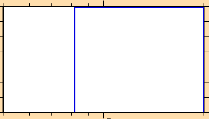
\sigma vs. E for ^{90}\text{Rb}(n,nt)
