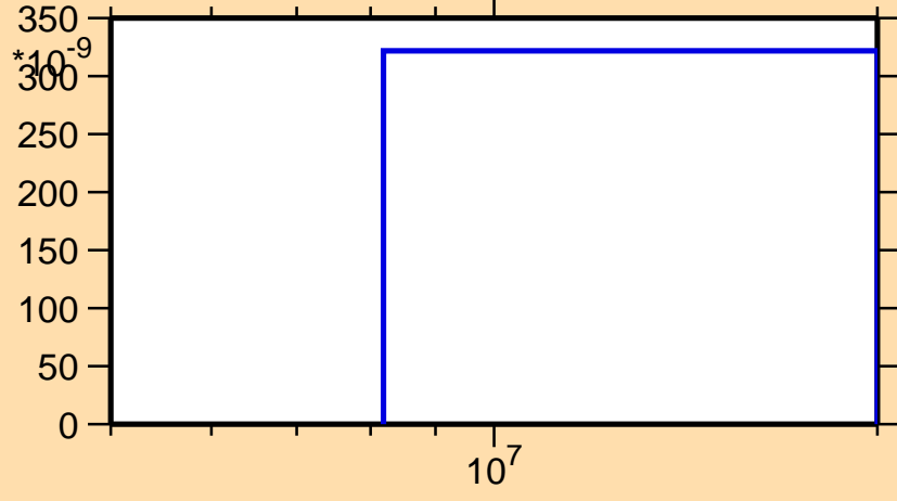
\sigma vs. E for ^{90}\text{Rb}(n,\text{nd})
