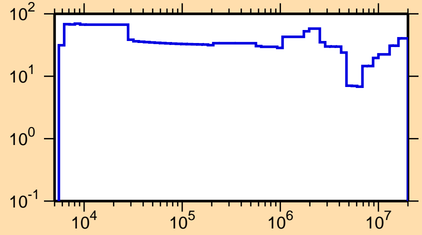
\Delta\sigma/\sigma vs. E for ^{92}\text{Rb}(n,\text{el.})
