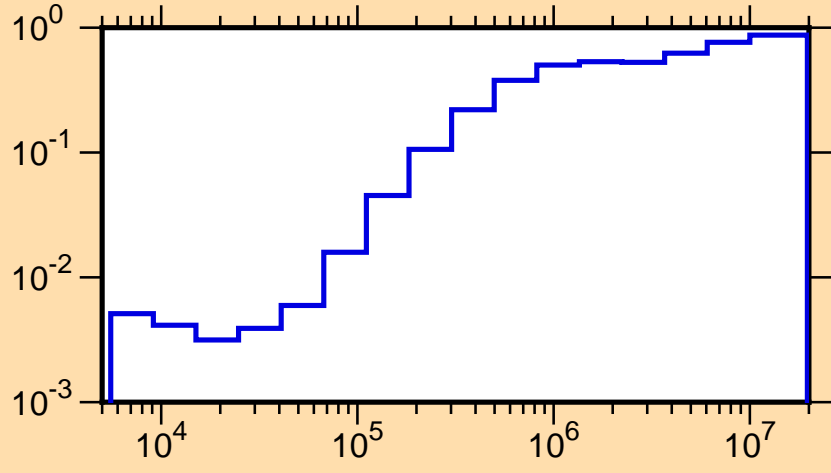
\mu vs. E for ^{92}\text{Rb}(\text{mt251})
