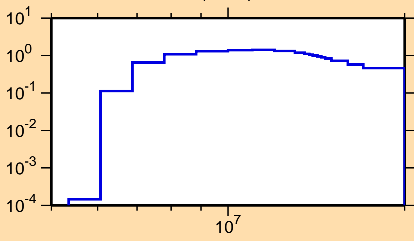
\sigma vs. E for ^{93}\text{Rb}(n,2n)
