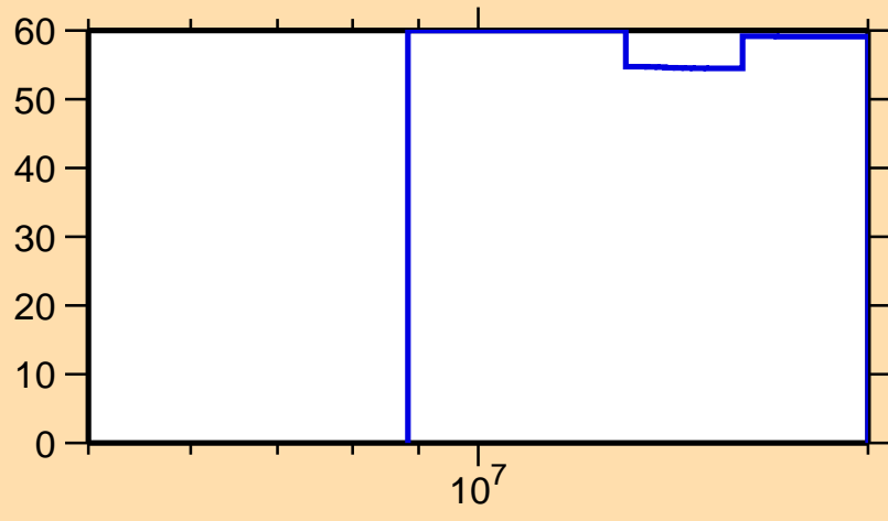
\Delta\sigma/\sigma vs. E for ^{93}\text{Rb}(n,p)
