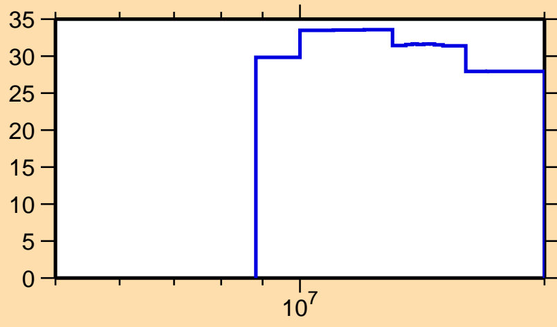
\Delta\sigma/\sigma vs. E for ^{93}\text{Rb}(n,ncont.)
