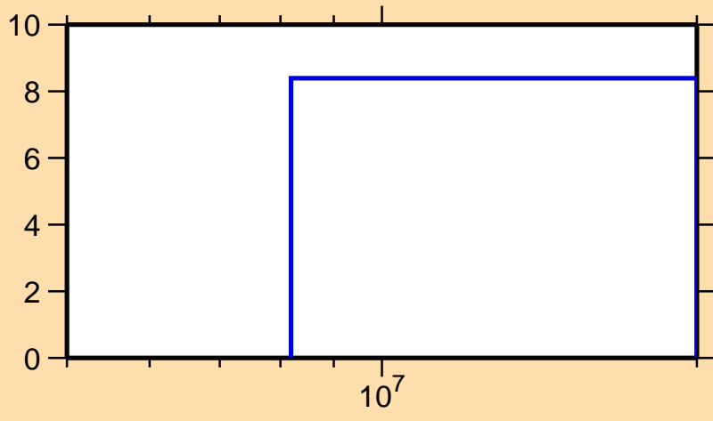
\Delta\sigma/\sigma vs. E for ^{93}\text{Rb}(n,el.)
