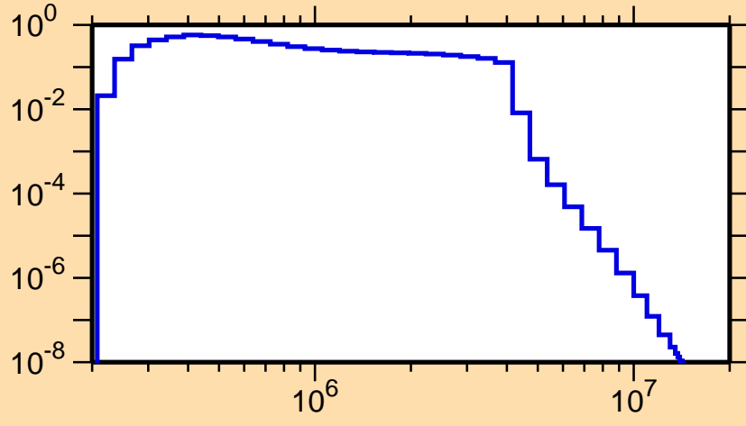
\sigma vs. E for ^{94}\text{Rb}(n,n_3)
