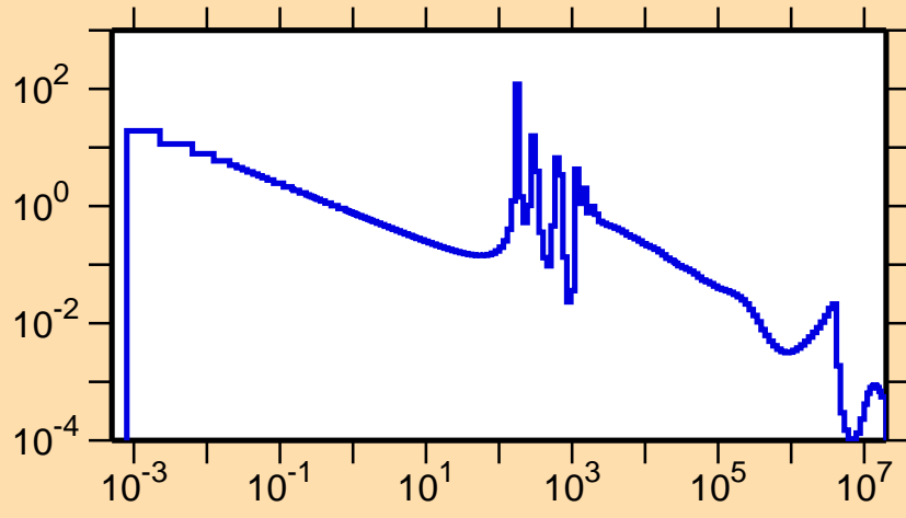
\sigma vs. E for ^{94}\text{Rb}(n,\gamma)
