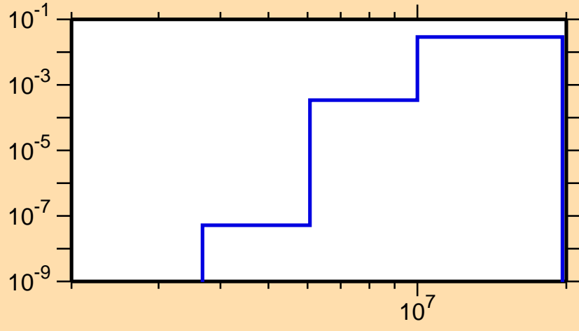
\sigma vs. E for ^{165}\text{Re}(\text{mt } 45)
