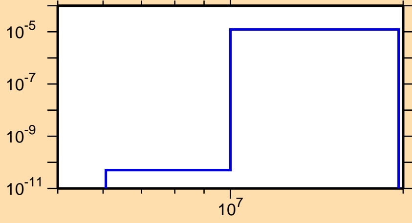
\sigma vs. E for ^{165}\text{Re}(n,\text{pd})
