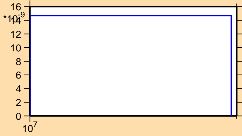
\sigma vs. E for ^{165}\text{Re}(n,\text{pt})
