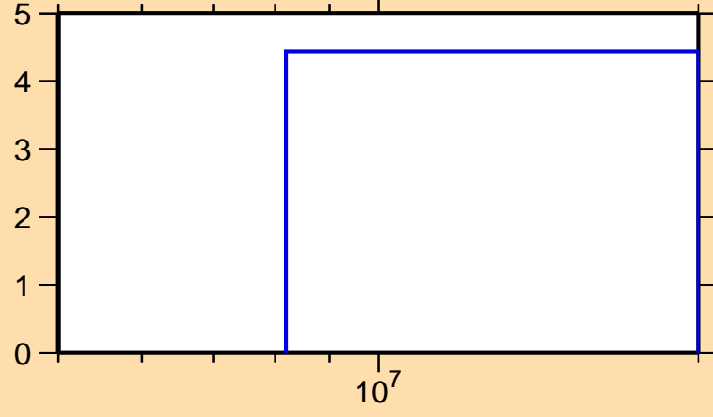
\Delta\sigma/\sigma vs. E for ^{165}\text{Re}(n,\text{el.})
