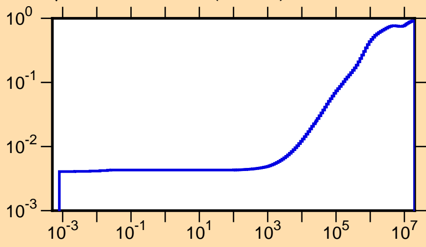
\mu vs. E for ^{166}\text{Re}(\text{mt251})
