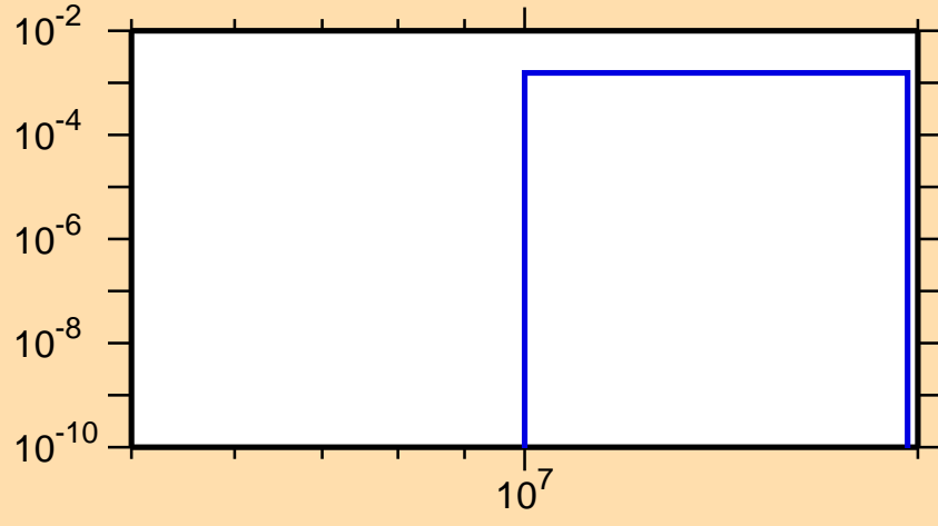
\sigma vs. E for ^{166}\text{Re}(n,2n\alpha)
