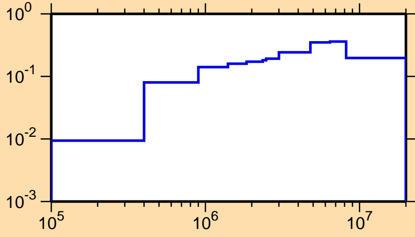
\sigma vs. E for ^{166}\text{Re}(n,n\text{cont.})
