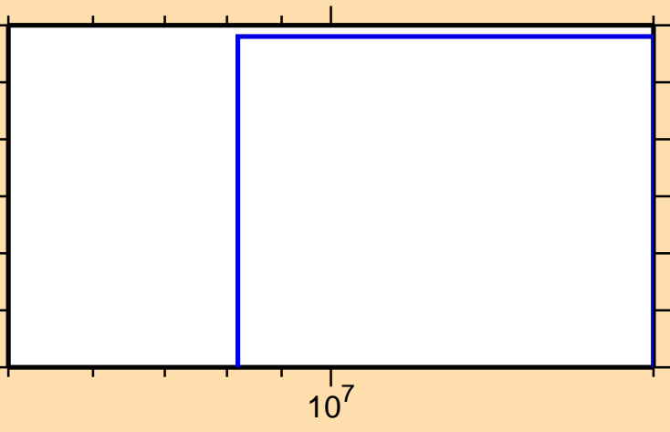
\sigma vs. E for ^{166}\text{Re}(n,2n)
