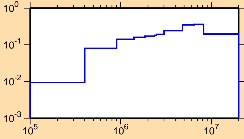
\sigma vs. E for ^{166}\text{Re}(n,\text{inel.})
