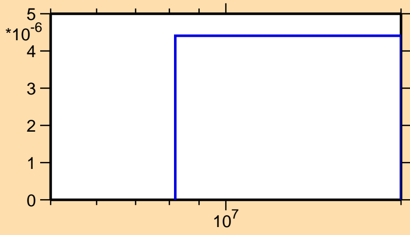
\sigma vs. E for ^{166}\text{Re}(n,\text{nd})
