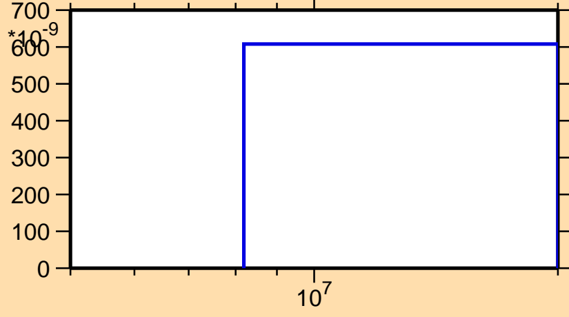
\sigma vs. E for ^{166}\text{Re}(n,\text{pt})
