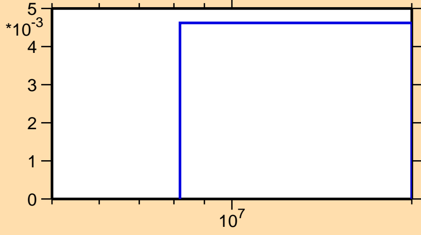
\sigma vs. E for ^{166}\text{Re}(n,2np)
