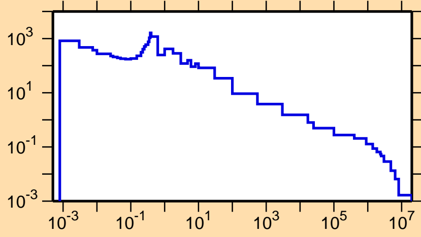
\sigma vs. E for ^{166}\text{Re}(n,\gamma)
