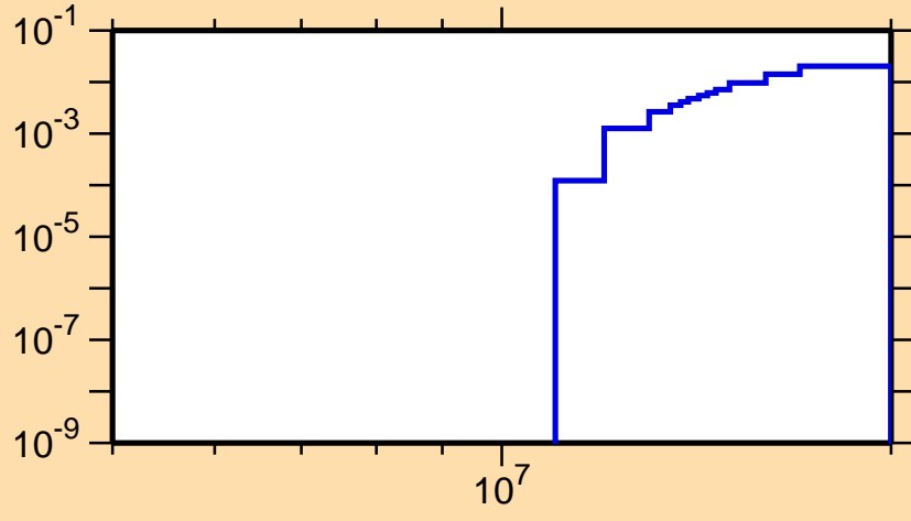
\sigma vs. E for ^{167}\text{Re}(n,2n\alpha)
