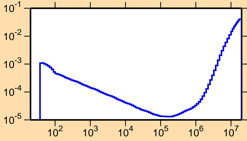
\sigma vs. E for ^{167}\text{Re}(n, p\alpha)
