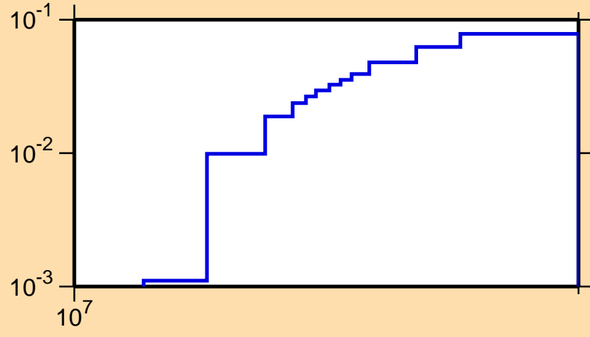
\sigma vs. E for ^{167}\text{Re}(n,2n)
