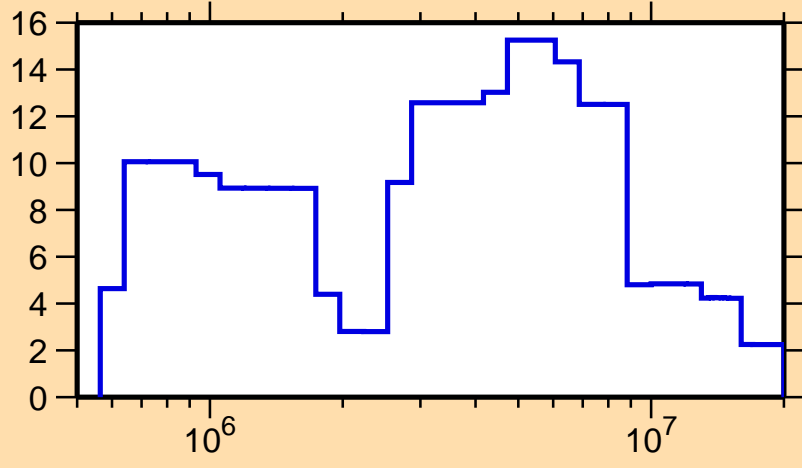
\Delta\sigma/\sigma vs. E for ^{167}\text{Re}(n,\text{tot.})
