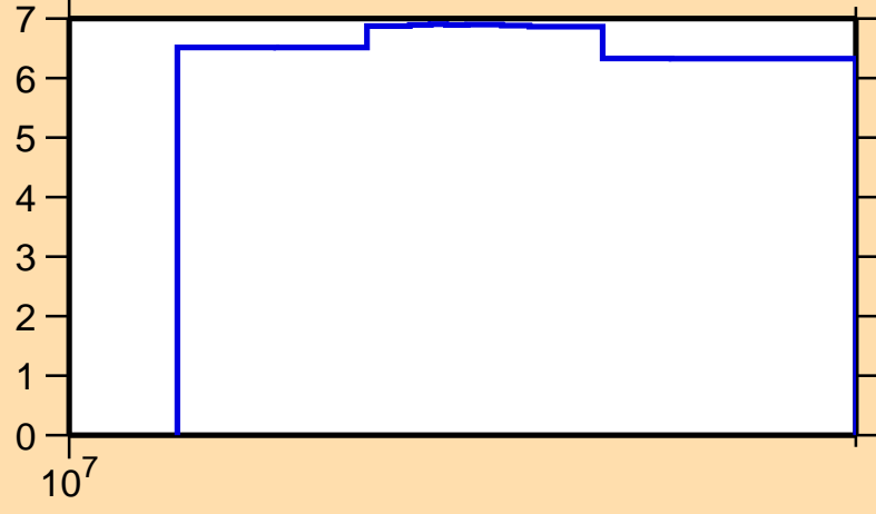
\Delta\sigma/\sigma vs. E for ^{167}\text{Re}(n,\text{nonel.})
