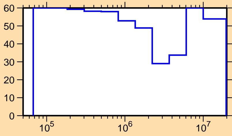
\Delta\sigma/\sigma vs. E for ^{167}\text{Re}(n,n_1)
