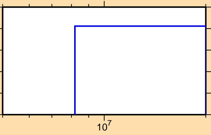
\sigma vs. E for ^{167}\text{Re}(n,2n\alpha)
