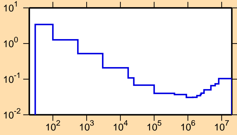
\sigma vs. E for ^{167}\text{Re}(n,\alpha)
