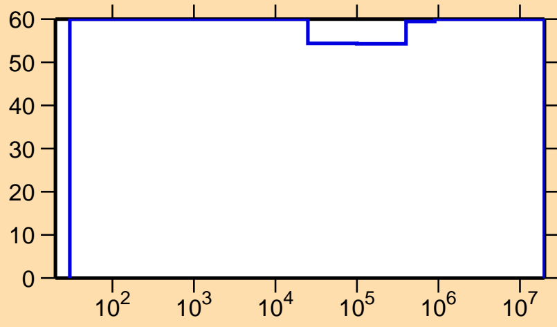
\Delta\sigma/\sigma vs. E for ^{167}\text{Re}(n,\gamma)
