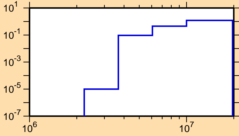
\sigma vs. E for ^{169}\text{Re}(n,np)
