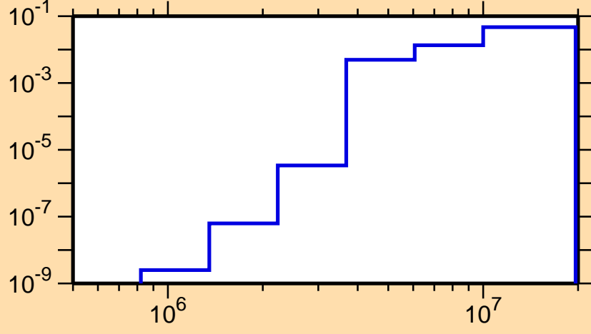
\sigma vs. E for ^{169}\text{Re}(n,n\alpha)
