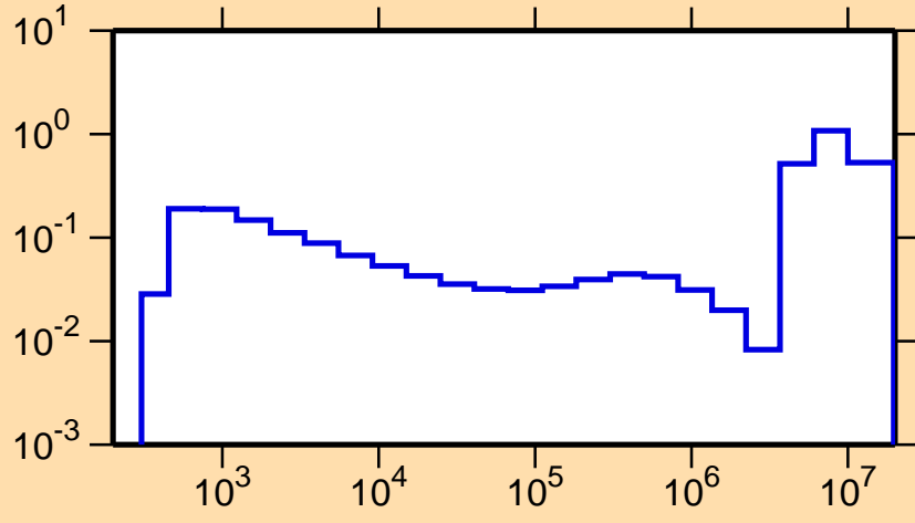
\sigma vs. E for ^{169}\text{Re}(n,\text{inel.})
