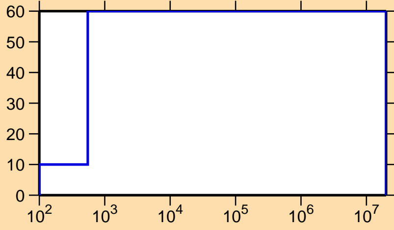
\Delta\sigma/\sigma vs. E for ^{169}\text{Re}(n,\gamma)
