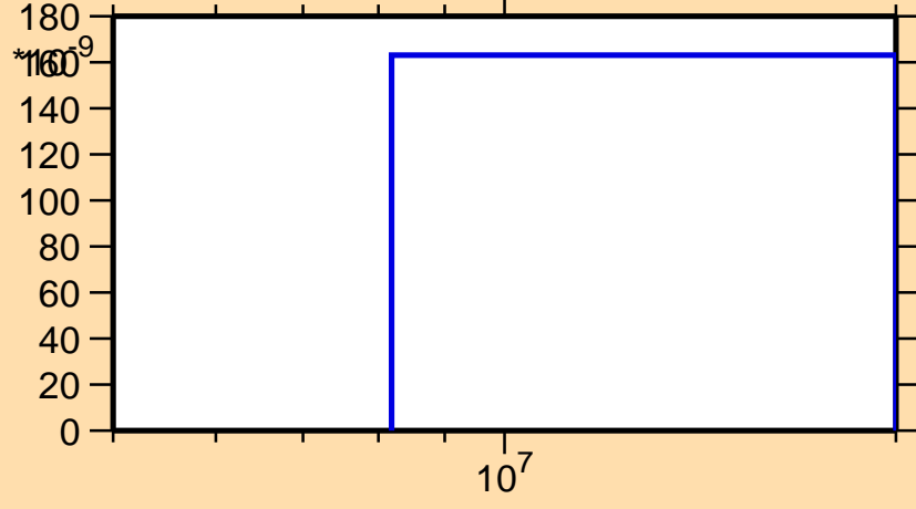
\sigma vs. E for ^{169}\text{Re}(n,\text{nd})
