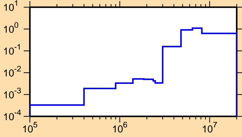
\sigma vs. E for ^{169}\text{Re}(n,n\text{cont.})
