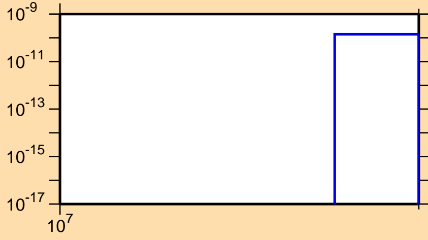
\sigma vs. E for ^{170}\text{Re}(n,3n\alpha)
