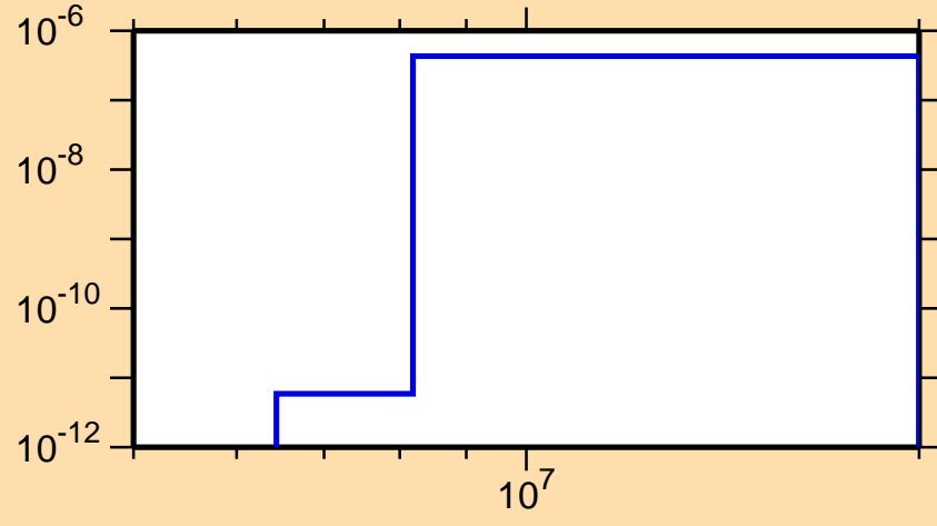
\sigma vs. E for ^{170}\text{Re}(\text{mt117})
