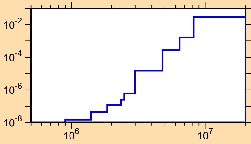
\sigma vs. E for ^{170}\text{Re}(n,n\alpha)
