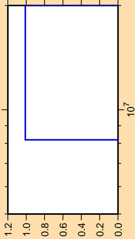
\Delta\sigma/\sigma vs. E for ^{170}\text{Re}(n,3n\alpha)
