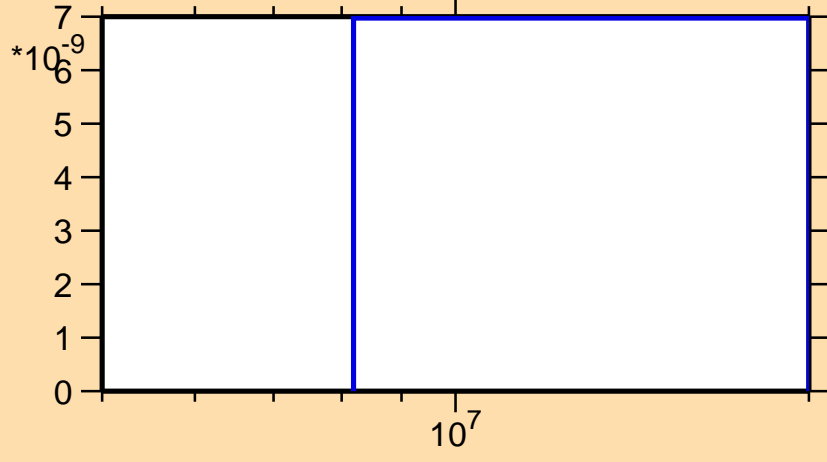
\sigma vs. E for ^{170}\text{Re}(n,\text{pt})
