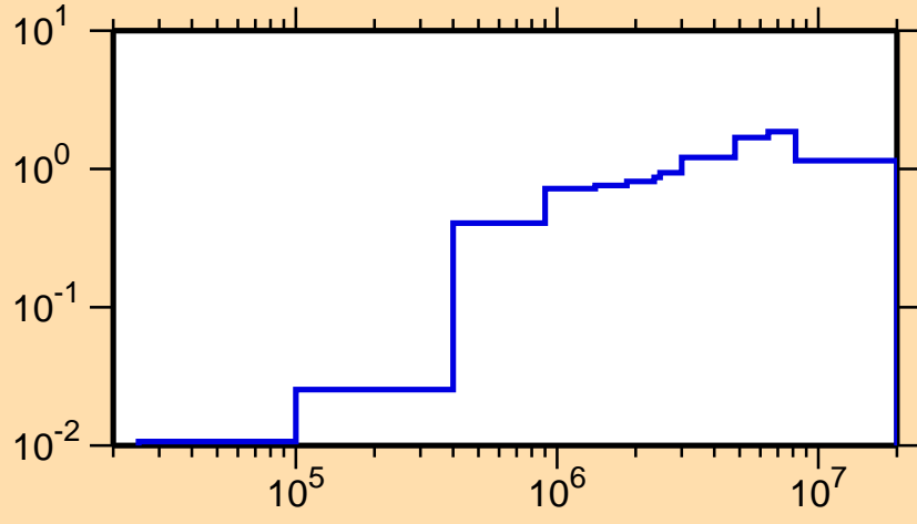
\sigma vs. E for ^{170}\text{Re}(n,\text{inel.})
