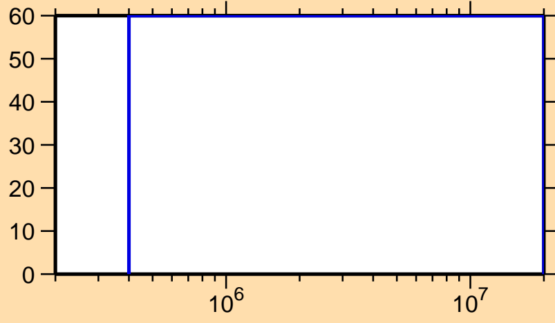
\Delta\sigma/\sigma vs. E for ^{170}\text{Re}(n,n\text{cont.})
