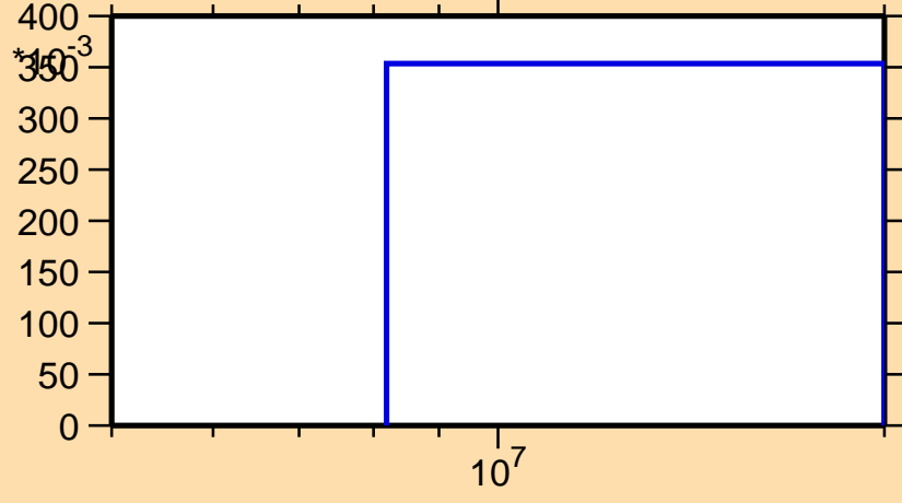
\sigma vs. E for ^{170}\text{Re}(n,2n)
