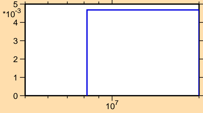
\sigma vs. E for ^{170}\text{Re}(n,2np)
