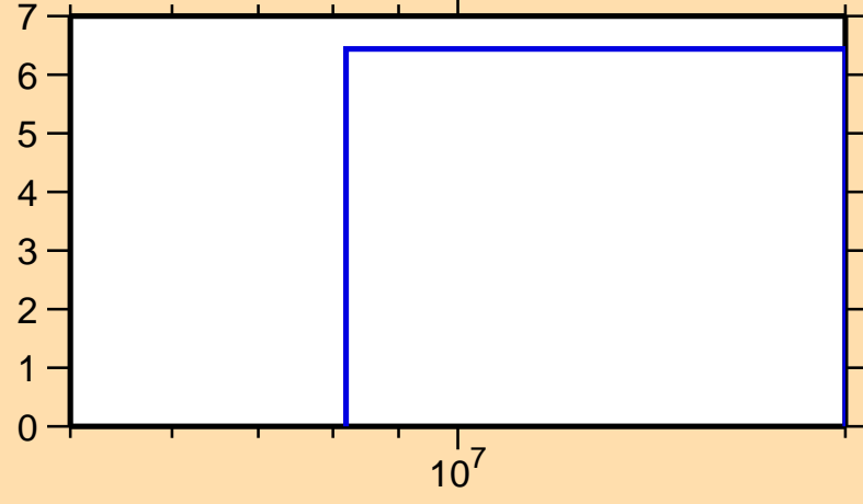
\Delta\sigma/\sigma vs. E for ^{170}\text{Re}(n,\text{nonel.})
