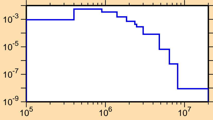
\sigma vs. E for ^{170}\text{Re}(n,n_4)
