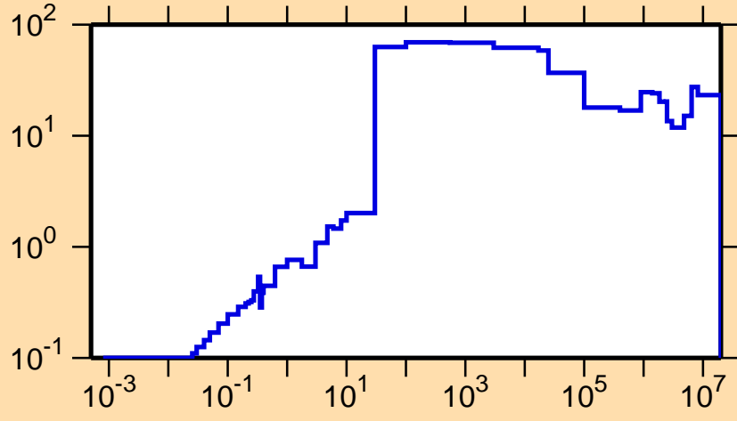
\Delta\sigma/\sigma vs. E for ^{170}\text{Re}(n,\text{tot.})
