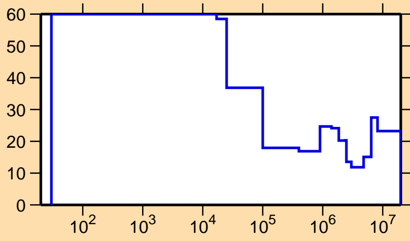
\Delta\sigma/\sigma vs. E for ^{170}\text{Re}(n,\text{tot.})
