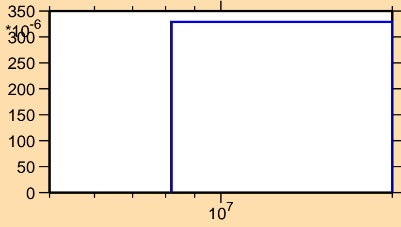
\sigma vs. E for ^{170}\text{Re}(n,2n\alpha)
