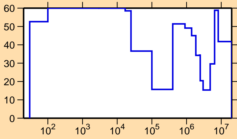
\Delta\sigma/\sigma vs. E for ^{170}\text{Re}(n,\text{el.})
