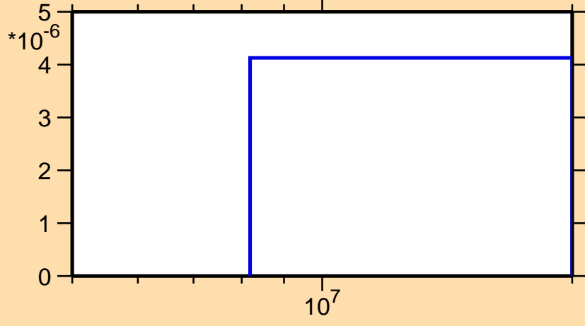
\sigma vs. E for ^{170}\text{Re}(n,\text{nd})
