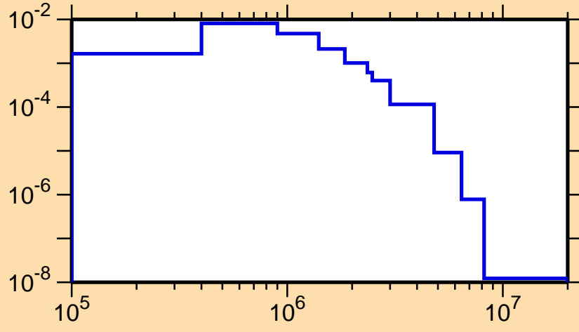
\sigma vs. E for ^{170}\text{Re}(n,n_3)
