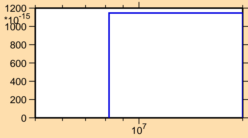
\sigma vs. E for ^{170}\text{Re}(n,3n\alpha)
