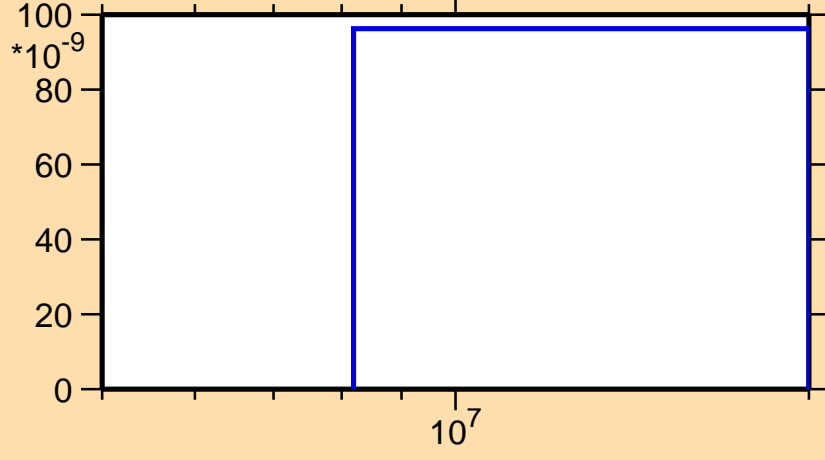
\sigma vs. E for ^{170}\text{Re}(n,\text{pd})
