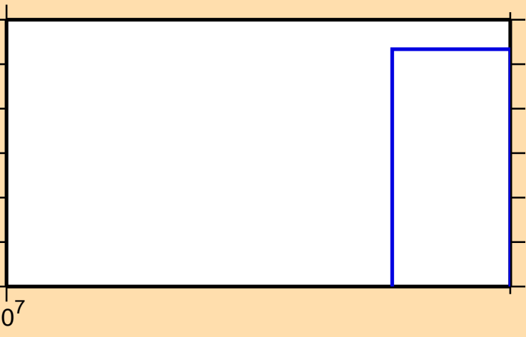
\sigma vs. E for ^{171}\text{Re}(n,3n)
