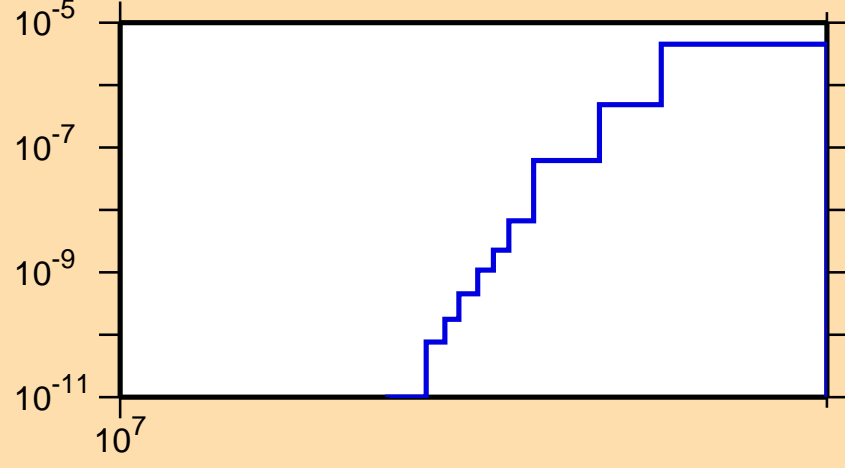
\sigma vs. E for ^{171}\text{Re}(n,\text{nd})
