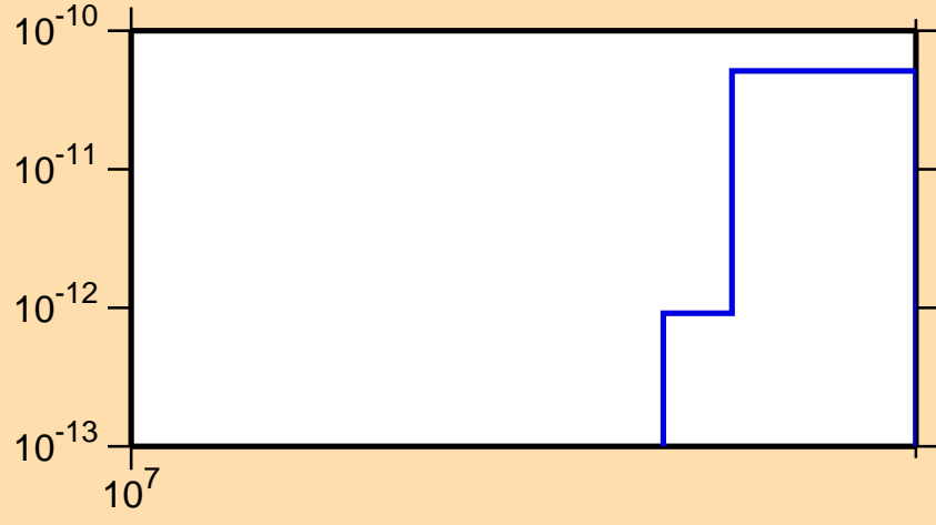
\sigma vs. E for ^{171}\text{Re}(\text{mt } 34)
