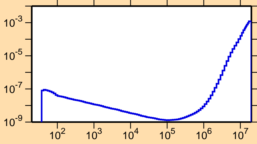
\sigma vs. E for ^{171}\text{Re}(n,p\alpha)
