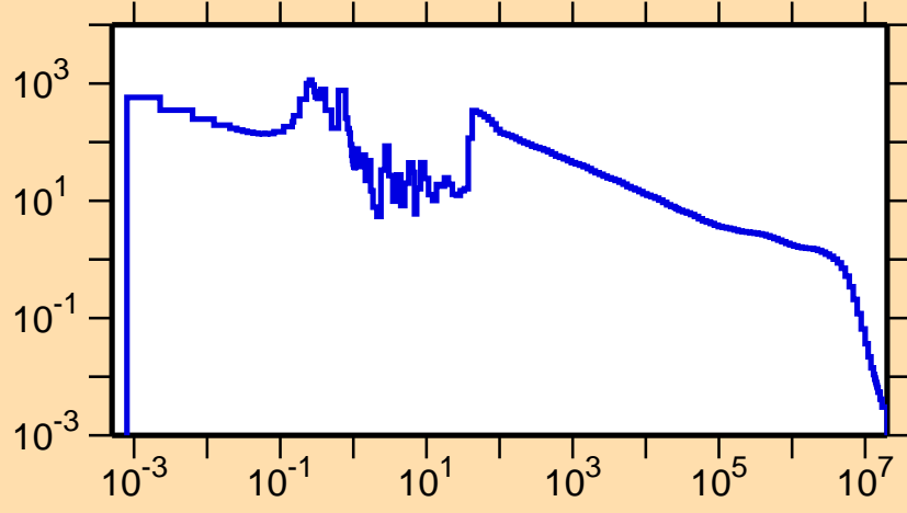
\sigma vs. E for ^{171}\text{Re}(n,\gamma)
