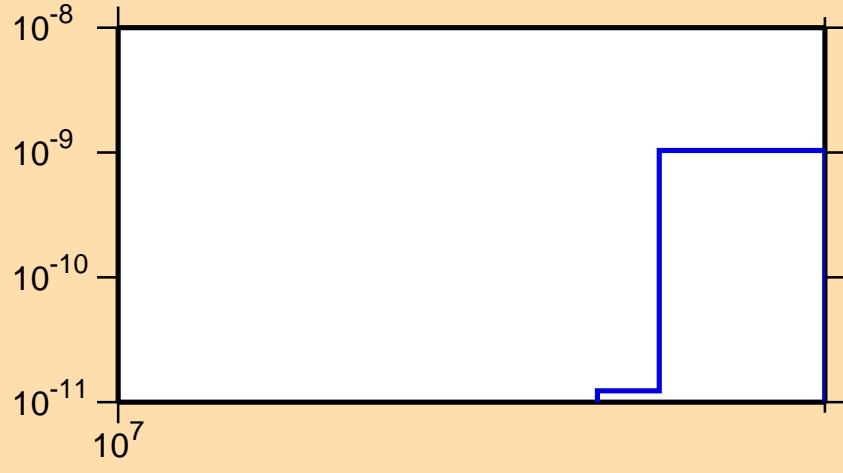
\sigma vs. E for ^{171}\text{Re}(n,\text{pt})
