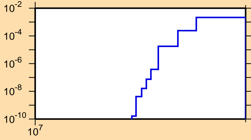
\sigma vs. E for ^{171}\text{Re}(n,2np)
