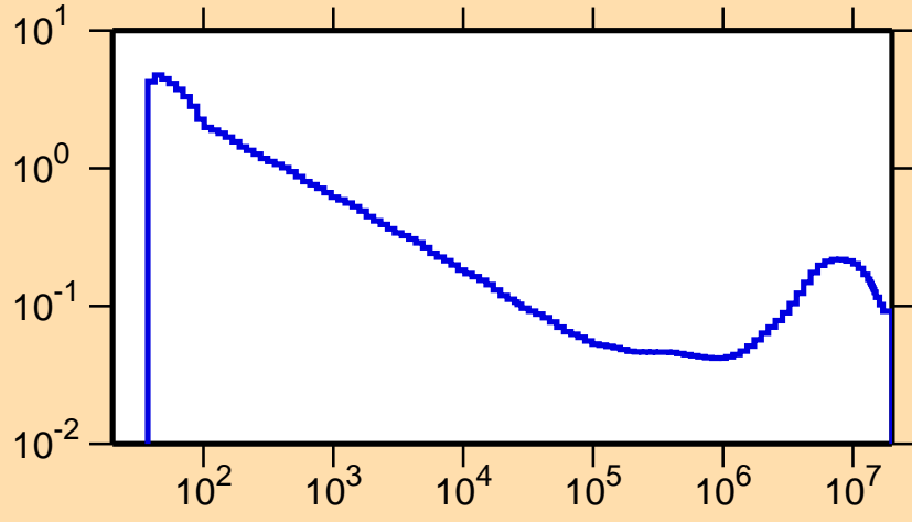
\sigma vs. E for ^{171}\text{Re}(n,p)
