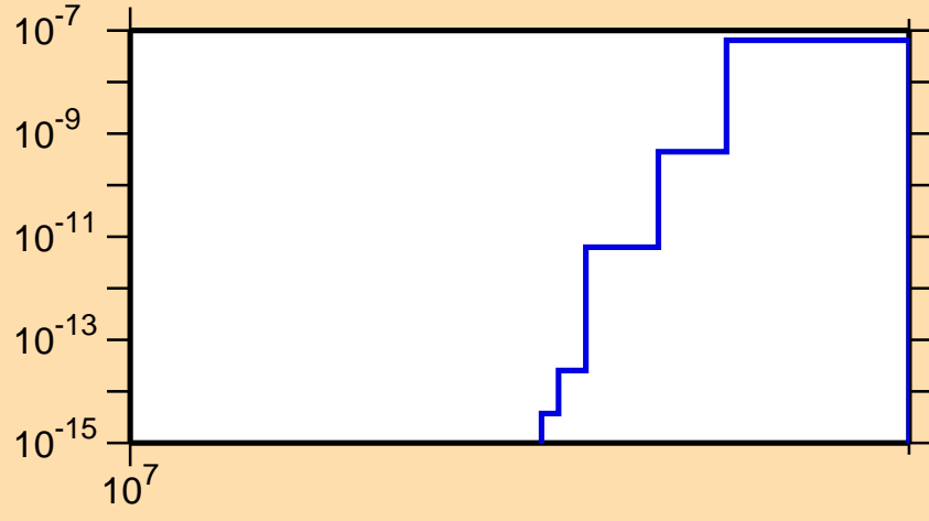
\sigma vs. E for ^{171}\text{Re}(n,nt)
