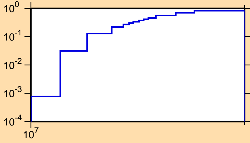
\sigma vs. E for ^{171}\text{Re}(n,2n)
