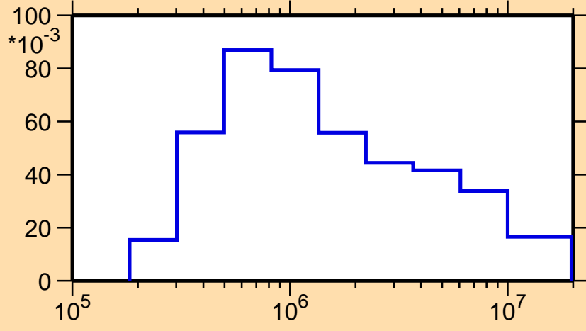
\sigma vs. E for ^{171}\text{Re}(n,n_2)
