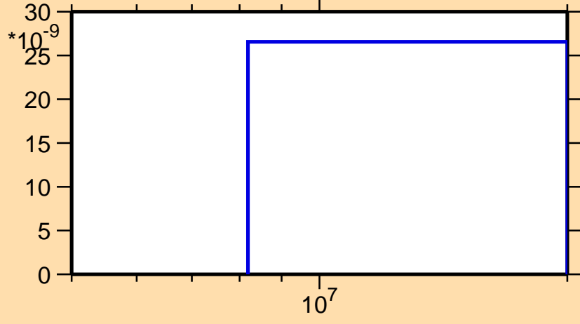
\sigma vs. E for ^{171}\text{Re}(n,\text{pd})
