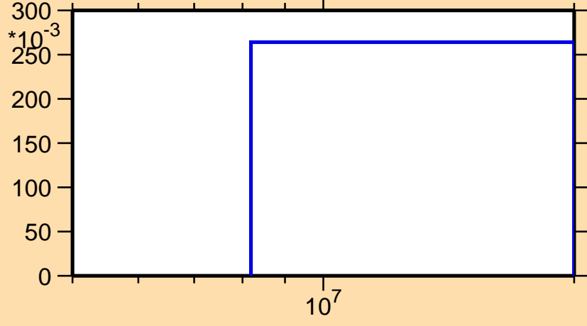
\sigma vs. E for ^{171}\text{Re}(n,2n)
