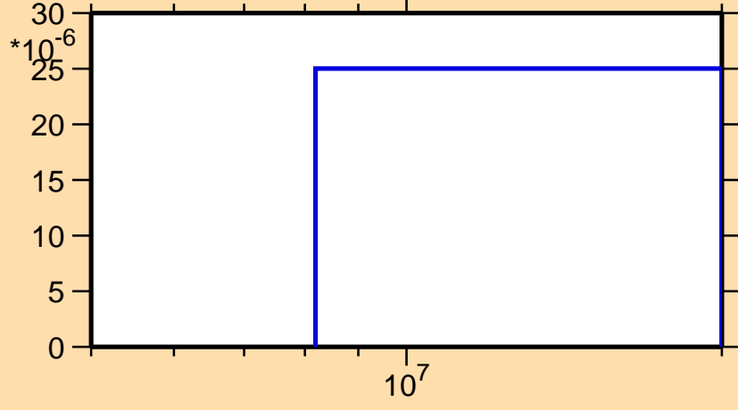
\sigma vs. E for ^{171}\text{Re}(n,2n\alpha)
