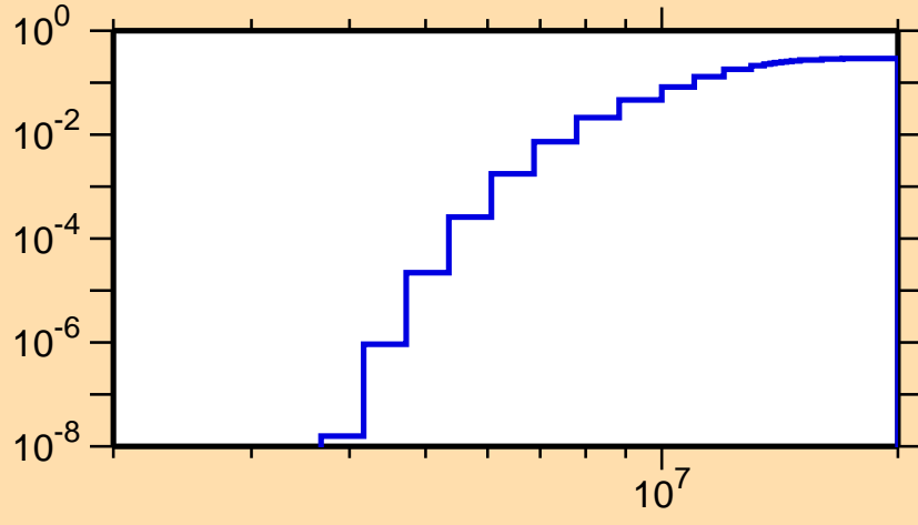
\sigma vs. E for ^{172}\text{Re}(n,np)
