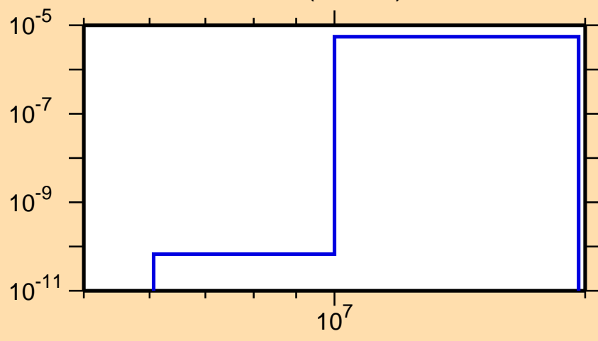
\sigma vs. E for ^{172}\text{Re}(n,\text{He3})
