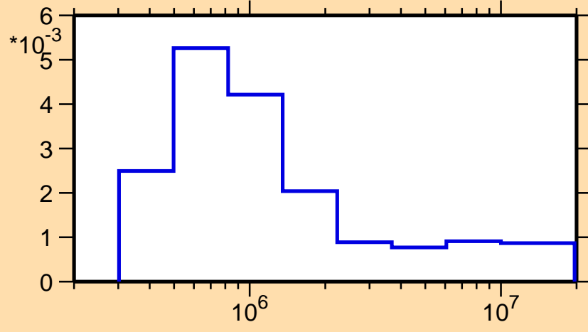
\sigma vs. E for ^{172}\text{Re}(n,n_4)
