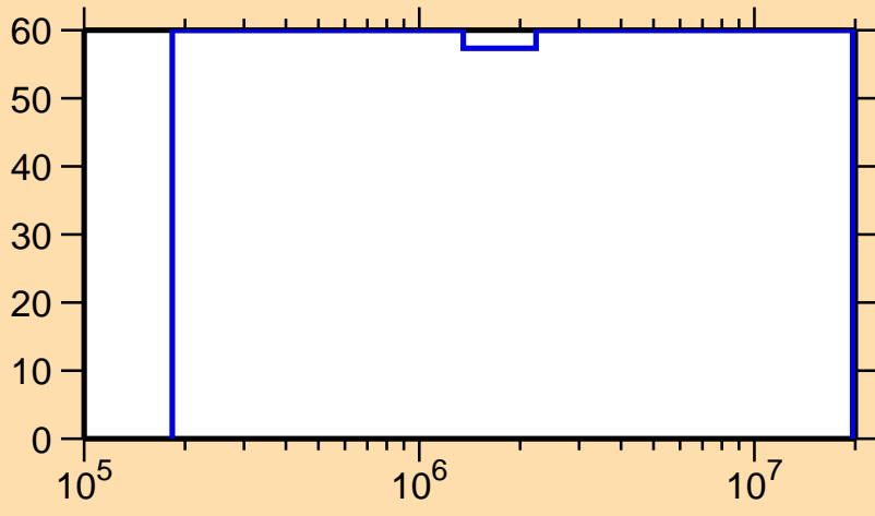
\Delta\sigma/\sigma vs. E for ^{172}\text{Re}(n,n_1)
